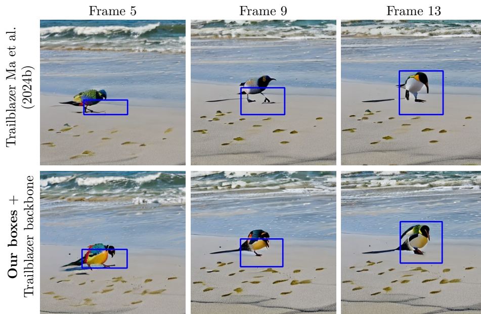
Figure 14: Additional qualitative results for morphing task (Parrot \rightarrow Penguin) – We show transition frames, where our optimized boxes provide benefit for better control of the morphing task.
