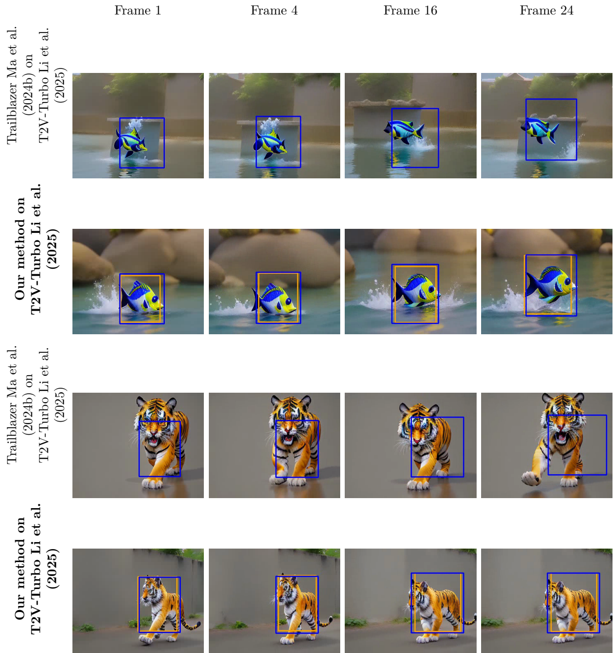
Figure 10: Additional qualitative results with T2V-Turbo Li et al. (2025) backbone – We show additional examples of our edits. Ours show more consistency with user intent and is of higher quality within the box. The prompt for the top 2 rows is "The surgeonfish is swimming" , while the prompt for the bottom 2 rows is "The tiger is walking" . Video results are also available in the supplementary local HTML page.
