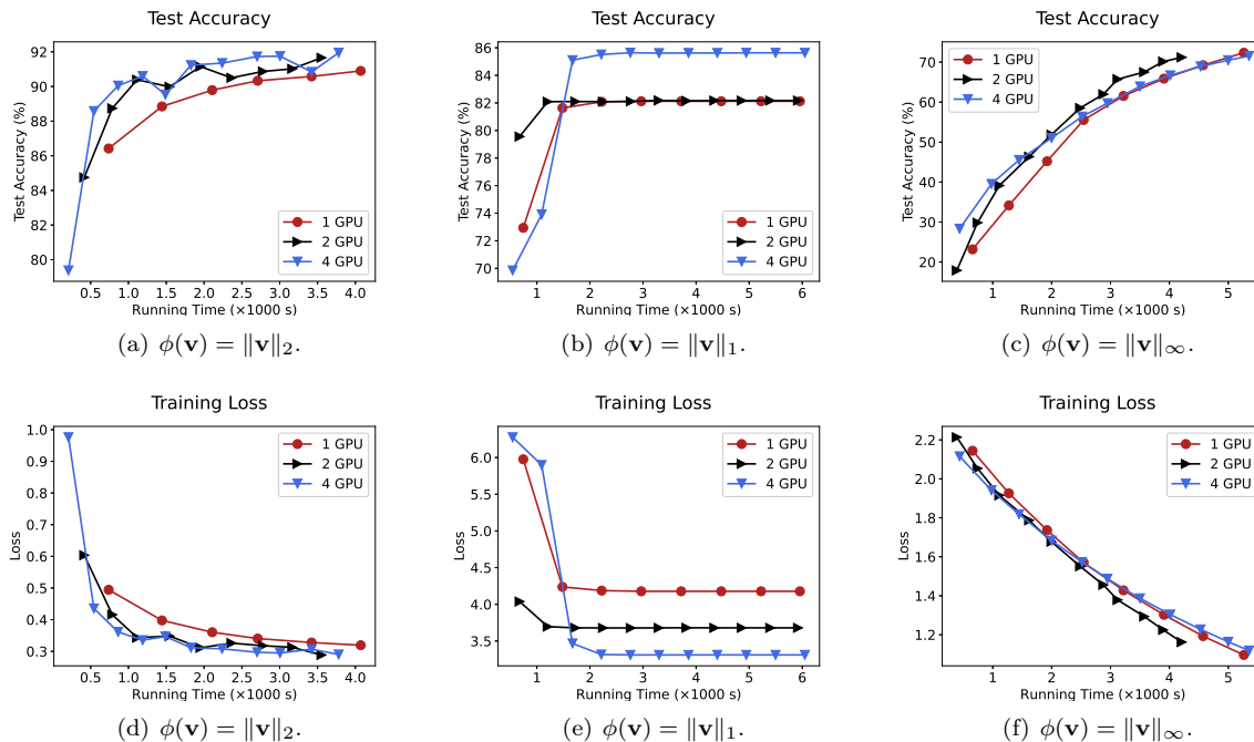
Figure 9: Testing Accuracy vs. running time (seconds) on MNIST of HD via Parallel Picard Iteration (Algorithm 5) under the cases of different forms of kinetic energy \phi(\cdot) .
