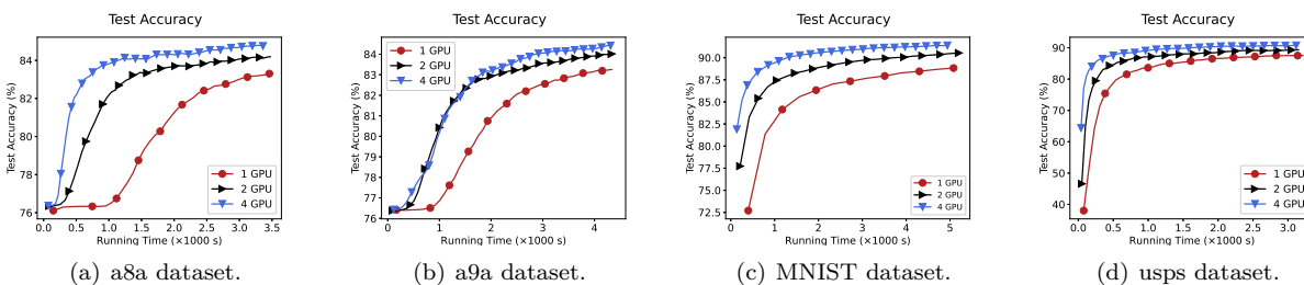
Figure 5: Testing accuracy vs. running time (seconds) on the four datasets of HD via Parallel Picard Iteration (Algorithm 5) with \phi(\mathbf{v}) = \frac{1}{2}\|\mathbf{v}\|_2^2 .
