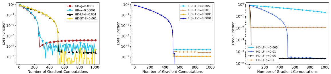
(a) Function value F(\cdot) vs. # gradient computations. (b) HDs with different step sizes \theta (integration time \eta fixed). (c) HDs with different values of integration time \eta (step size \theta fixed).
