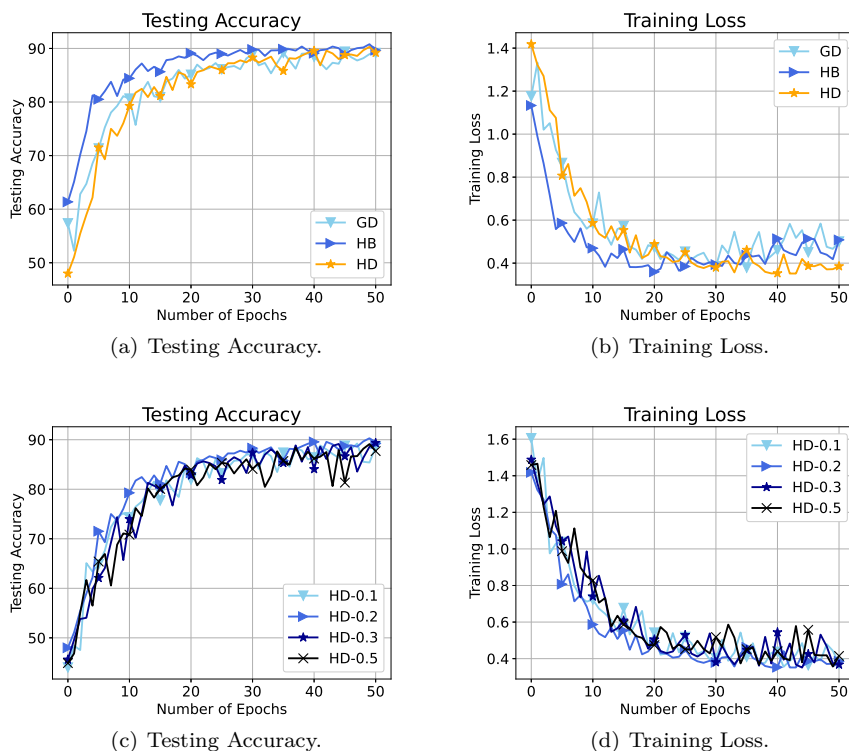
Figure 4: Testing Accuracy and Training Loss of neural network training with different algorithms and parameters.
