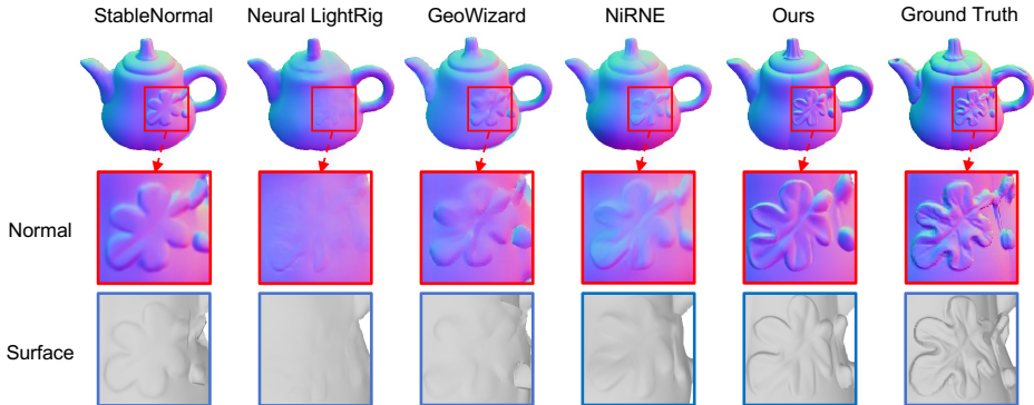
Figure 2: Illustration of 3D misalignment. The estimated normal maps of previous methods may appear to have an overall correct color distribution, yet the reconstructed surfaces often fail to align with the accurate geometry details, showing over-smooth results. Our estimated normal map has a higher 3D alignment compared to others.
