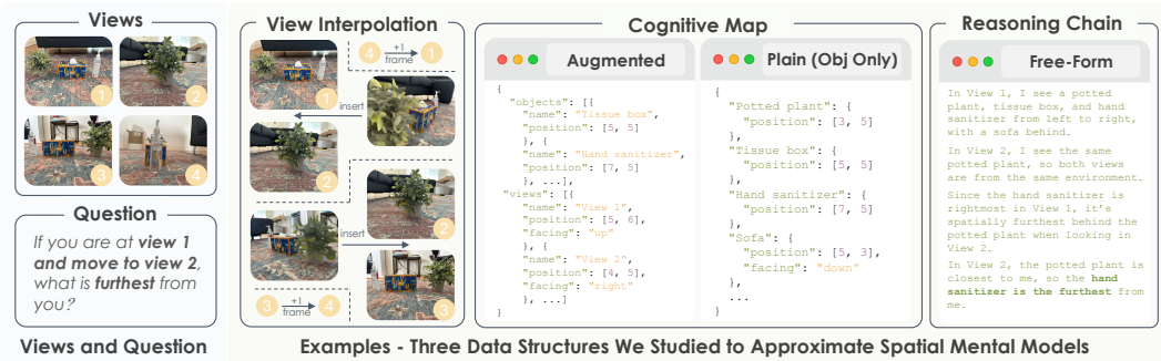
Figure 3: Grounded examples of our three data structures that approximate spatial mental models. effective. Drawing on this literature, we define three data structures below (detailed introduction can be found in Appendix D.1), each targeting distinct cognitive properties (integration, transformation, inference) of spatial mental models, with grounded examples in Figure 3:
