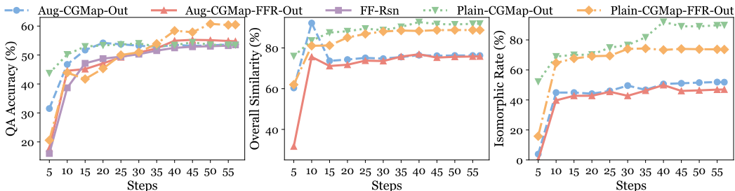
Figure 5: SFT training dynamics under fixed spatial object order. Compared to randomized order (Figure 4), the overall learning trends are consistent: Plain-CGMap-FFR-Out achieves the highest QA accuracy despite not producing the most structurally perfect maps.
