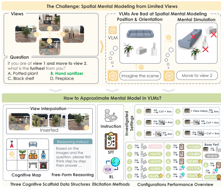
Figure 1: Top: VLMs cannot maintain a coherent mental model when evaluating on the MINDCUBE benchmark. Bottom: We study how we can help build spatial mental models through external (scaling of views, cognitive map input) and internal strategies (fine-tuning, cognitive map elicitation). We find joint cognitive map and reasoning setting yields the highest gain (+23.52%).
