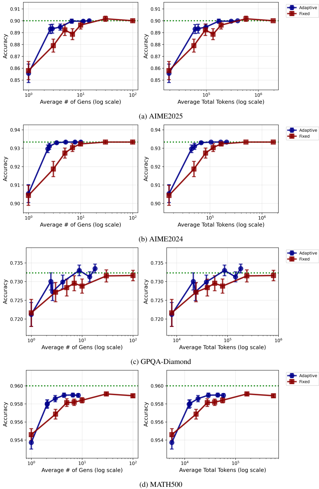
Figure 10: Cost-analysis of our proposed method and fixed BoN for Qwen3-30B-A3B-Thinking-2507. The error bars are standard two-sigma confidence intervals. Green dashed line indicates the best-of- \infty performance.
