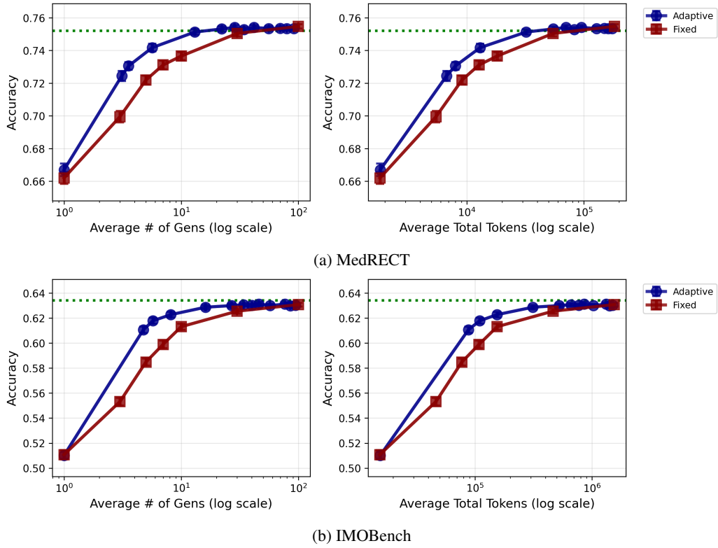
Figure 17: Cost-analysis of our proposed method and fixed BoN for GPT-OSS-20B. The error bars are standard two-sigma confidence intervals. Green dashed line indicates the best-of- \infty performance.
