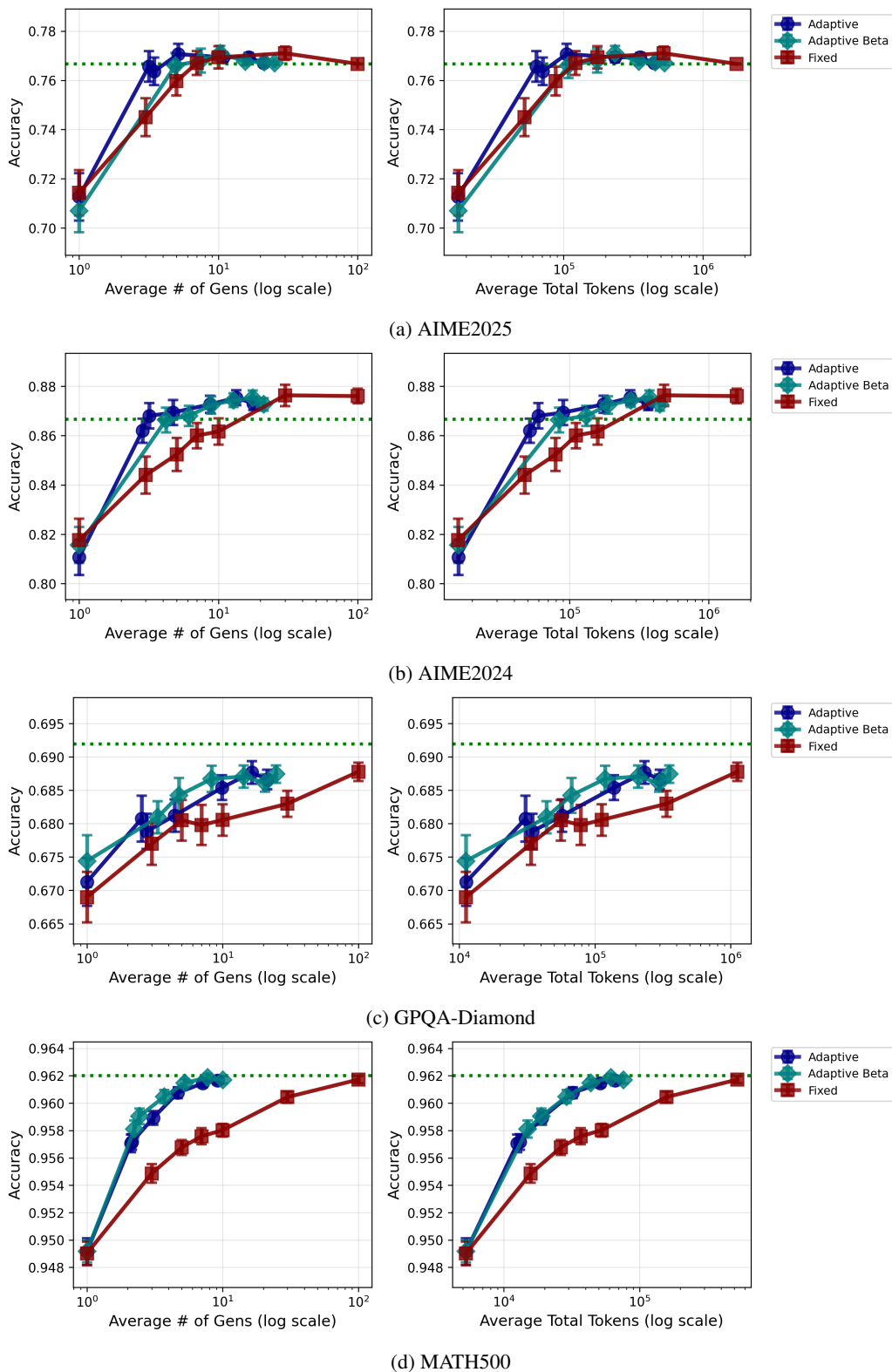
Figure 16: Cost-analysis of our proposed method (“adaptive”), Beta stopping (Aggarwal et al., 2023), and fixed BoN for EXAONE-Deep-32B. The error bars are standard two-sigma confidence intervals. Green dashed line indicates the best-of- \infty performance.
