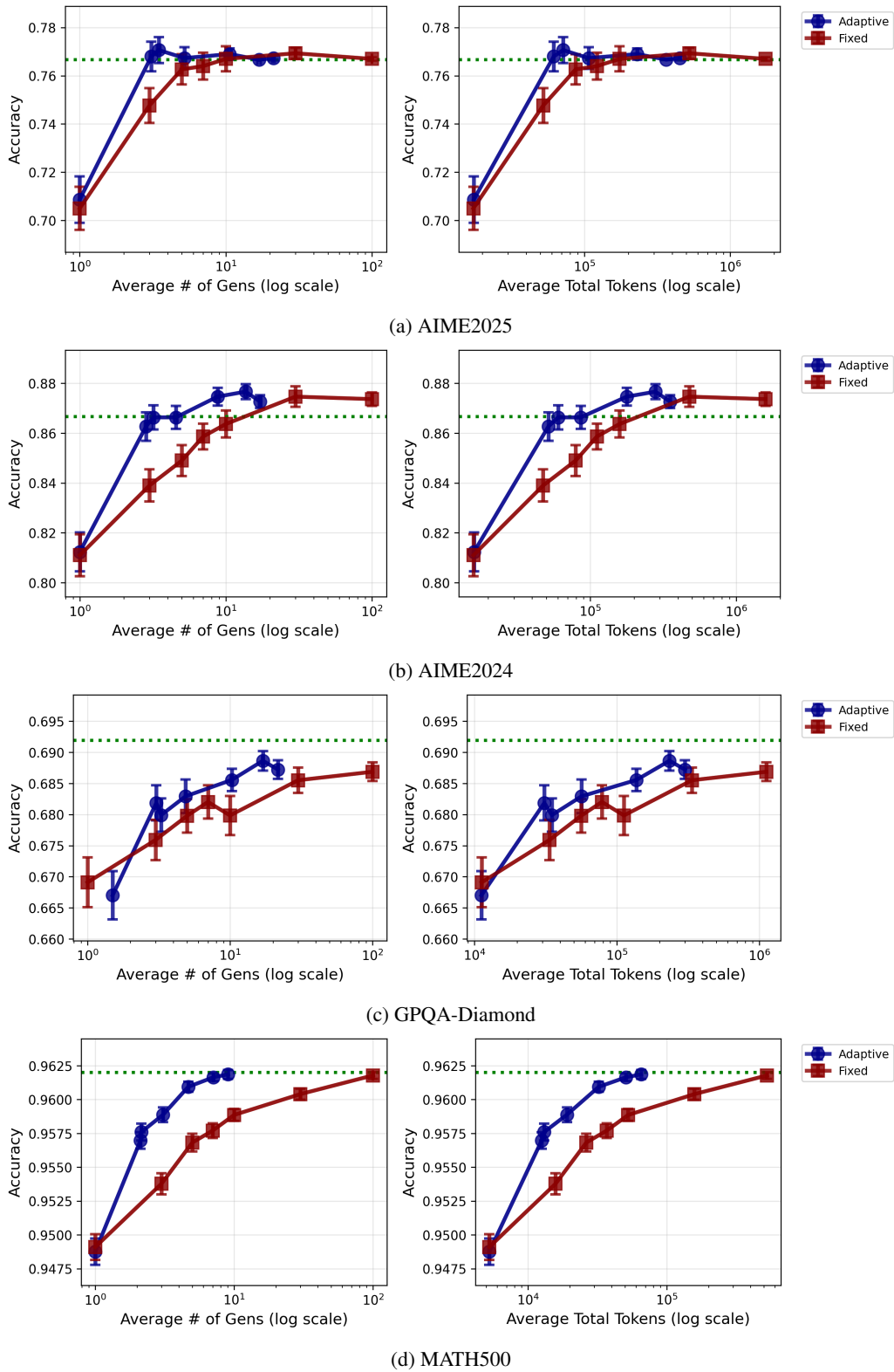
Figure 11: Cost-analysis of our proposed method and fixed BoN for EXAONE-Deep-32B. The error bars are standard two-sigma confidence intervals. Green dashed line indicates the best-of- \infty performance.
