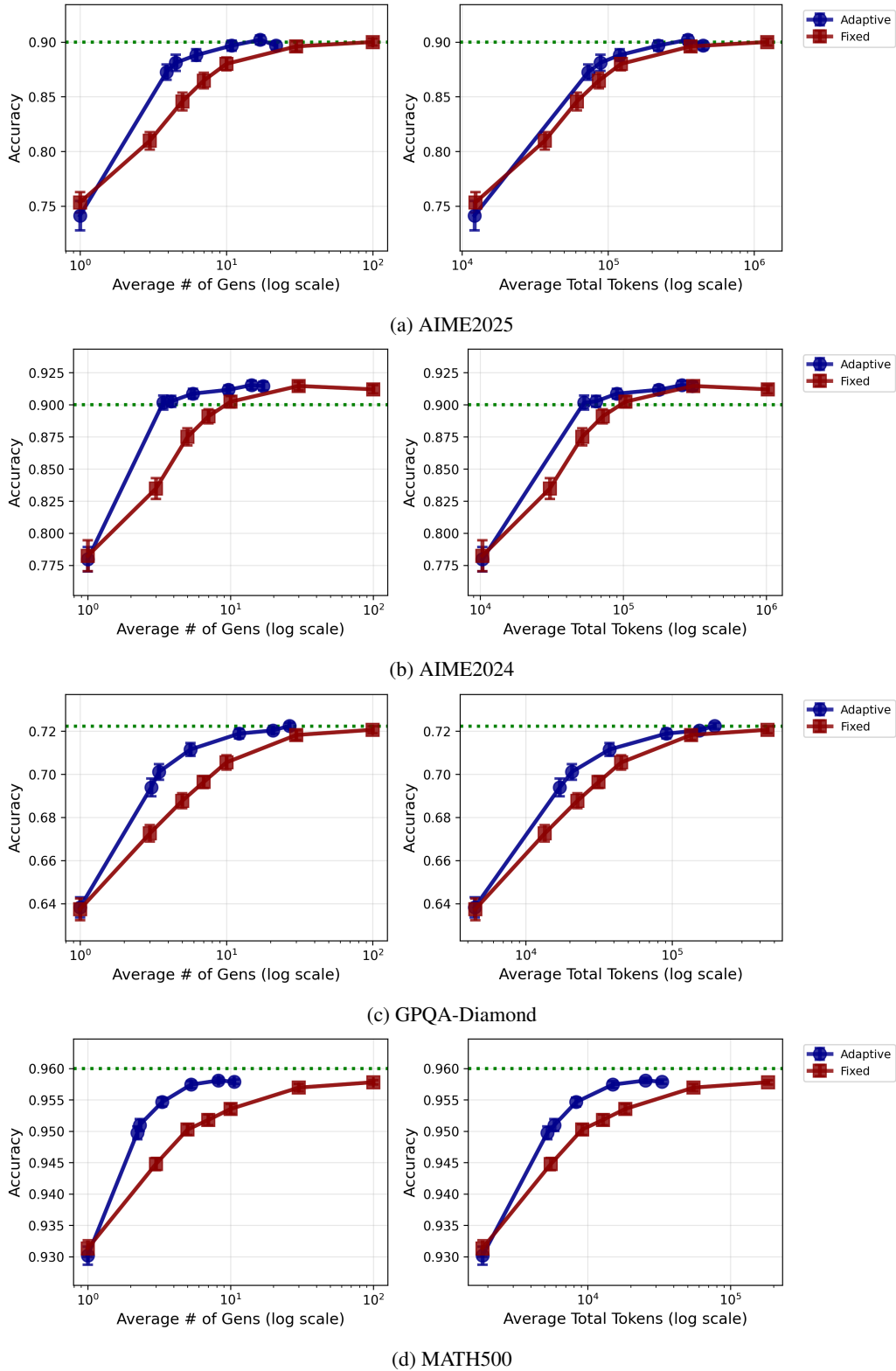
Figure 7: Cost-analysis of our proposed method and fixed BoN for GPT-OSS-20B. The error bars are standard two-sigma confidence intervals. Green dashed line indicates the best-of- \infty performance.
