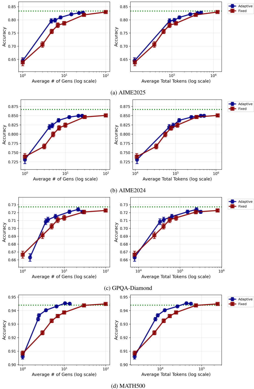
Figure 8: Cost-analysis of our proposed method and fixed BoN for Phi-4-reasoning. The error bars are standard two-sigma confidence intervals. Green dashed line indicates the best-of- \infty performance.
