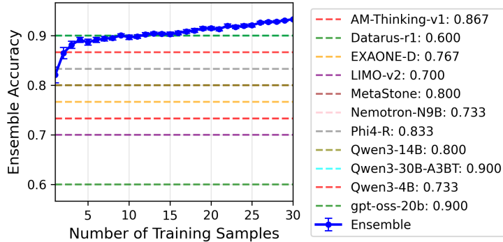
Figure 6: The number of samples to determine the weight (x-axis) as a performance of best-of- \infty (y-axis) on AIME2025. The x-axis indicates the number of problems used to learn the weight and the y-axis indicates the best-of- \infty performance with all problems. The score is averaged over 100 runs. The optimal weight has achieved the limit accuracy of 93.3%, whereas the best single LLM has the limit accuracy of 90.0%. Dashed lines indicate the best-of- \infty performance of each LLM.
