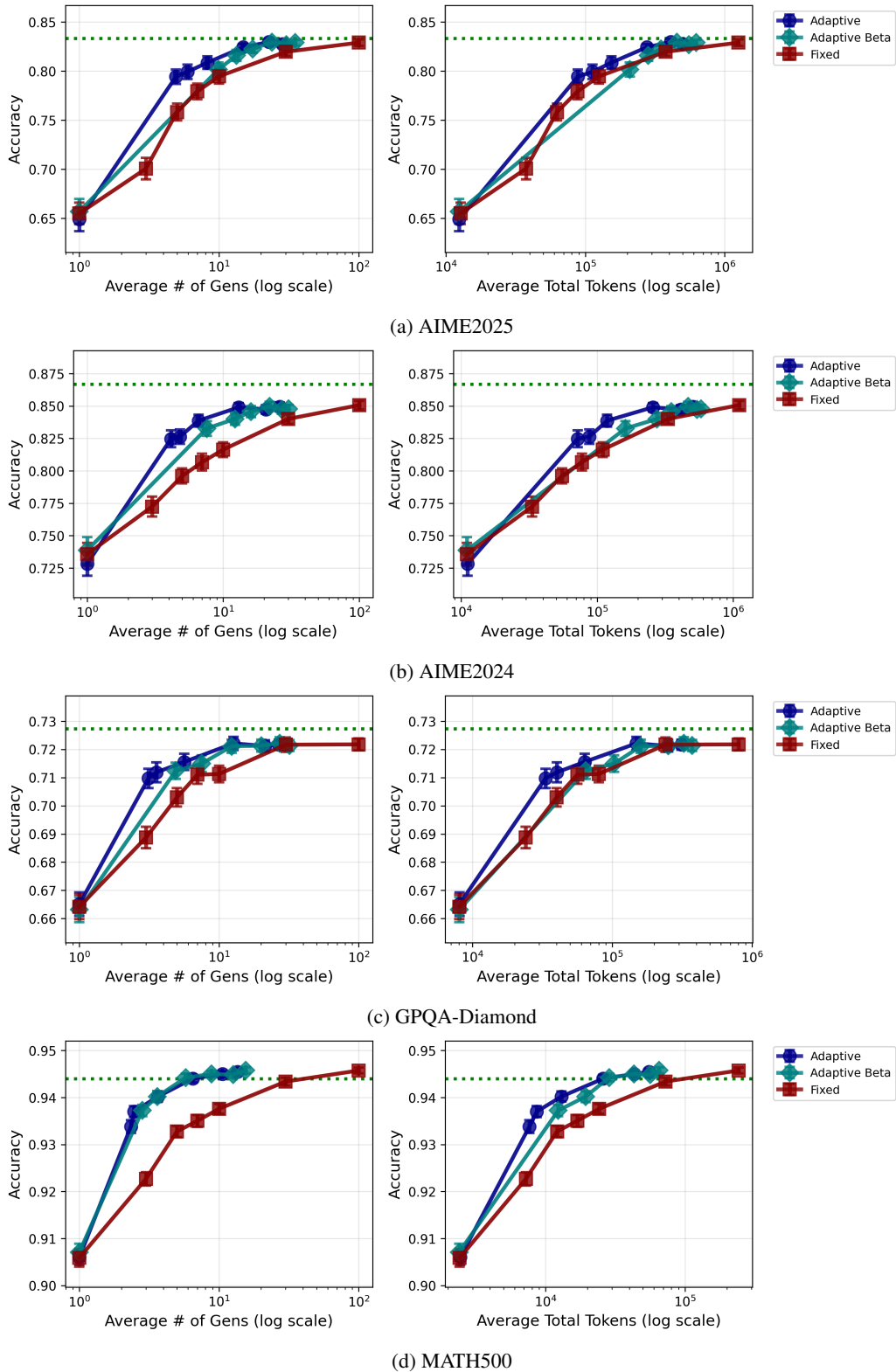
Figure 15: Cost-analysis of our proposed method (“adaptive”), Beta stopping (Aggarwal et al., 2023), and fixed BoN for Phi-4-reasoning. The error bars are standard two-sigma confidence intervals. Green dashed line indicates the best-of- \infty performance.
