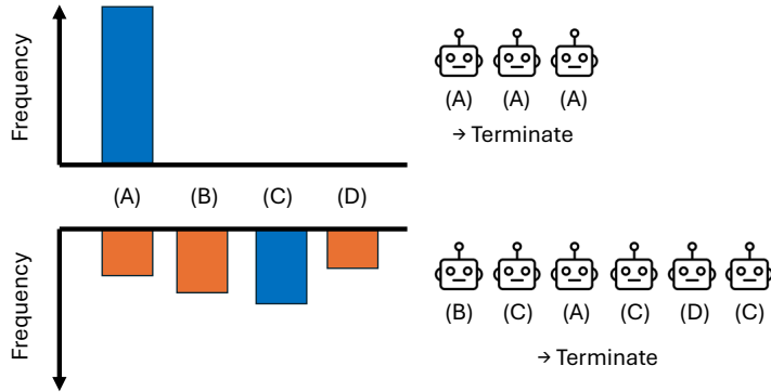
Figure 2: An illustration of adaptive sampling (Algorithm 1). The histogram shows the distribution of answers generated by an LLM for a single problem. Each answer generation can be viewed as a sample from the underlying distribution. Blue indicates the most frequent answer, and orange indicates the others. In the top example, three generations agree, so sampling stops. In the bottom example, more samples are needed to determine the majority. This maximizes the accuracy under a given compute budget. Confidence in the majority is based on the Bayes factor.
