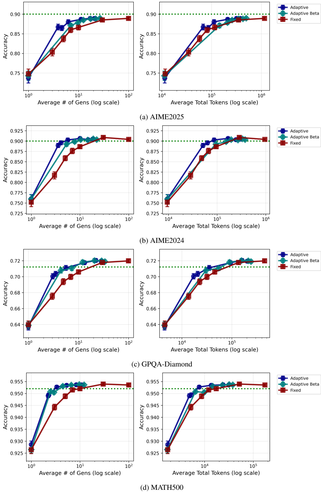
Figure 14: Cost-analysis of our proposed method (“adaptive”), Beta stopping (Aggarwal et al., 2023), and fixed BoN for GPT-OSS-20B. The error bars are standard two-sigma confidence intervals. Green dashed line indicates the best-of- \infty performance.
