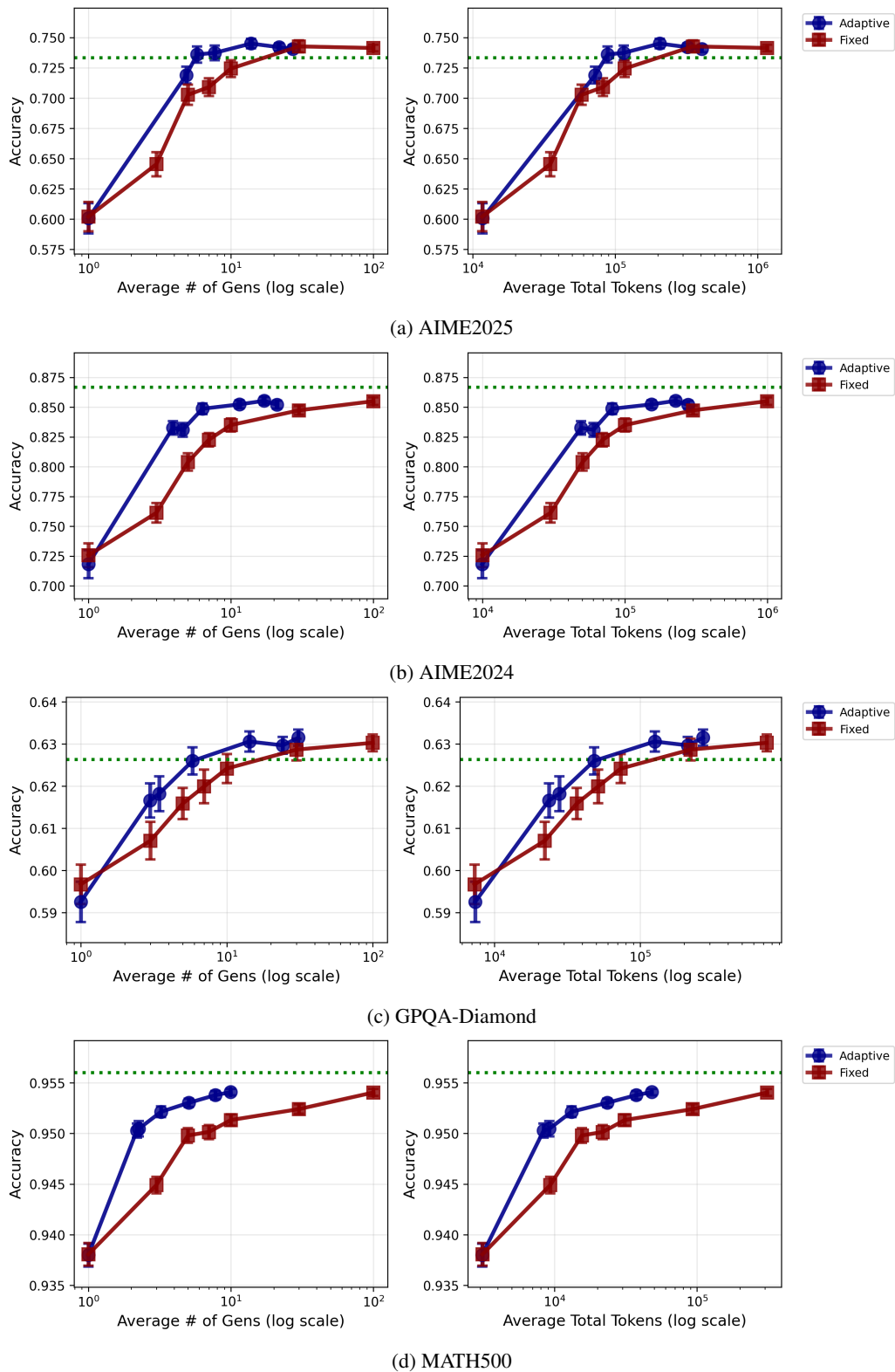
Figure 9: Cost-analysis of our proposed method and fixed BoN for NVIDIA-Nemotron-Nano-9B-v2. The error bars are standard two-sigma confidence intervals. Green dashed line indicates the best-of- \infty performance.
