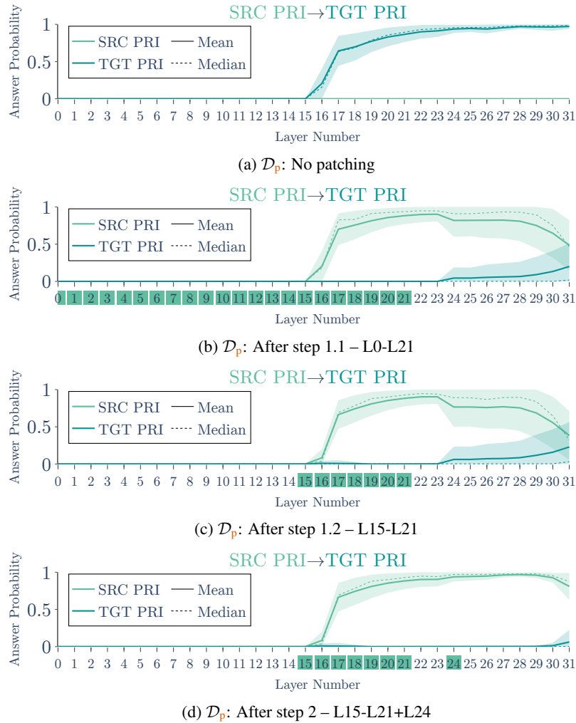
Figure 6: Visualization of the TIP at various stages of the search algorithm on Llama 3.1 Instruct FT 🍌. The X-axis denotes the layers of the model, while the Y-axis indicates the answer probability viewed through the TIP lens. (a) Displays the initial TIP before any patching is applied. (b) Shows the TIP after step 1.1, which identifies the end of the base range. (c) Illustrates the TIP following step 1.2, where the start of the base range is located. Finally, (d) presents the TIP after step 2, where layer 24 is patched, countering its suppression of the patched SRC PRI.
