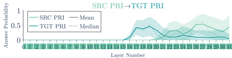
Figure 8: TIP of patching all MLP outputs on Llama 3.1 Instruct FT \blacklozenge with patching setup \mathcal{D}_p .
