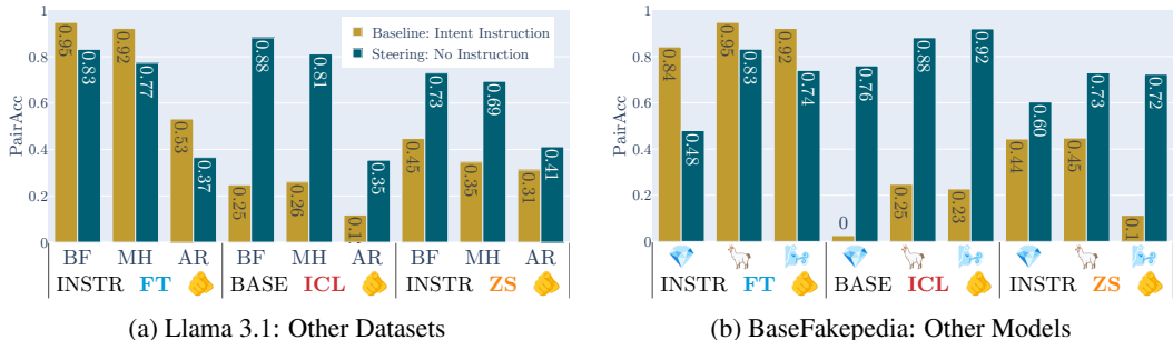
Figure 4: We compare pair accuracy of a baseline model (with intent instructions) against the steered model (without intent instructions). We consider baseline models: (i) instruct model fine-tuned on CCS-BF, (ii) base model with 10 in-domain ICL demonstrations, and (iii) the default instruct model. Left: Subspace steering on Llama 3.1 generalizes across datasets (BASEFAKEPEDIA (BF), MULTIHOPFAKEPEDIA (MF), and ARITHMETIC (AR)). Right: For multiple models (Llama 3.1 8b (🐼), Gemma 2 9b (🔹), and Mistral 7b v0.3 (🐝)), a rank-1 subspace can be used for effective steering.
