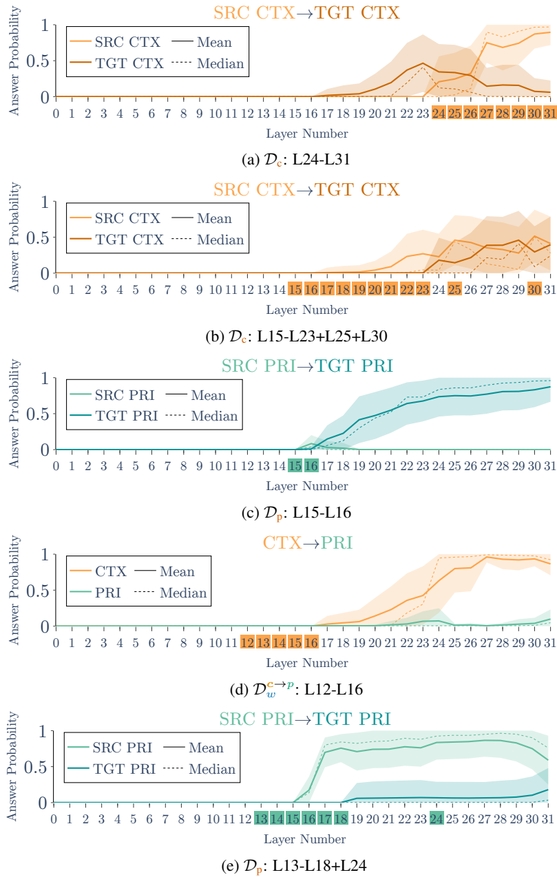
Figure 7: Additional TIP visualizations of answer probabilities across different patching settings on Llama 3.1 Instruct FT \blacklozenge . The x -axis represents the layers, and the y -axis displays the answer probability under the TIP. The first row of each plot visualizes the patching flow.
