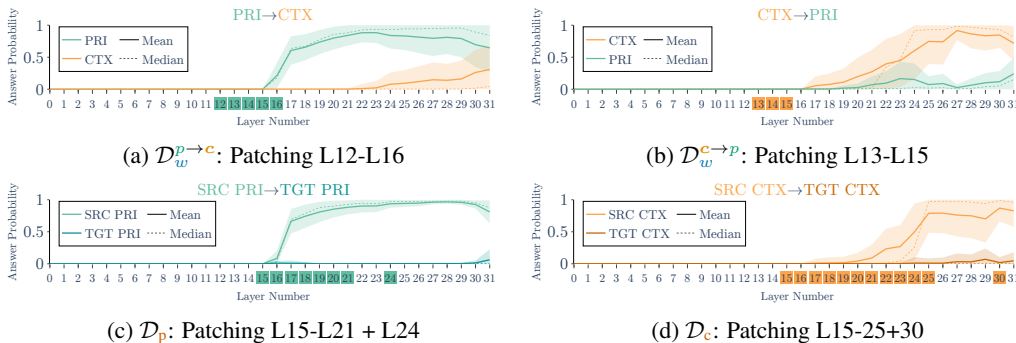
Figure 2: Answer probabilities per layer as determined by TIP for different patching settings on Llama 3.1 Instruct FT \clubsuit . The x -axis represents the layers. The y -axis shows the TIP answer probability. On the x -axis we mark the patched layers. Each row of subplots aims to answer one subquestion. Top Row: Where is w computed? Patching a source SRC PRI into a TGT CTX (left; 2a) and vice versa (right; 2b). Bottom Row: Where is a(q, \varepsilon) and a(q, c) computed? Patching a source SRC PRI into a TGT PRI, using samples from \mathcal{D}_p (2c) and the same for CTX (2d).
