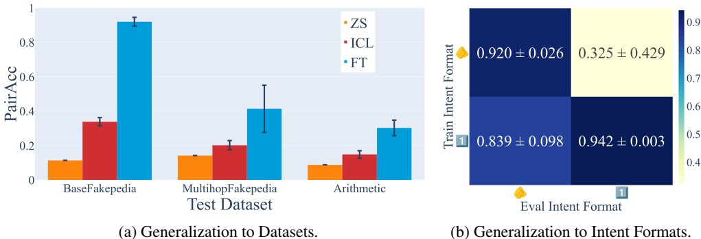
Figure 10: (a) Pair accuracy of Mistral-v0.3 7B-Instruct when evaluated on CCS-BF, CCS-MH, and CCS-AR datasets. For each dataset, we evaluate the model zero-shot, with 10 in-context learning examples from CCS-BF, and after fine-tuning on 2048 examples from CCS-BF. (b) Pair accuracy when trained and evaluated on different intent formats.
