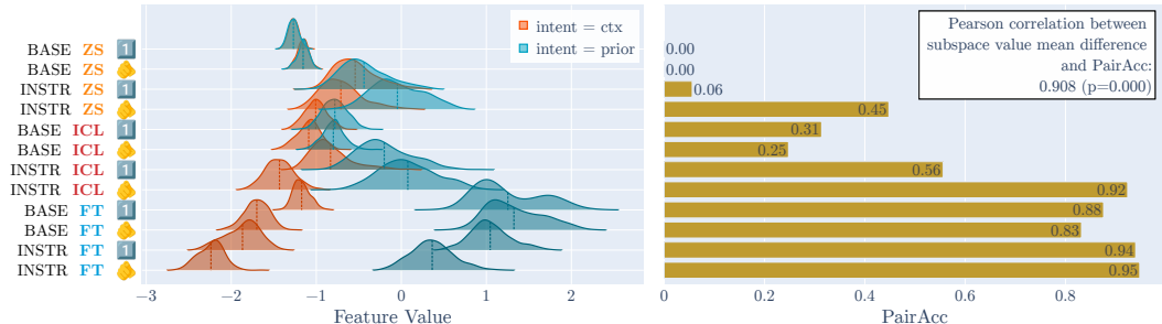
Figure 5: Subspace \mathcal{F}_w value distributions of different model configurations (left) and baseline model performance on CCS-BF (right). We can observe a high correlation between the absolute difference between the means of the two groups (ctx and pri) and the performances.
