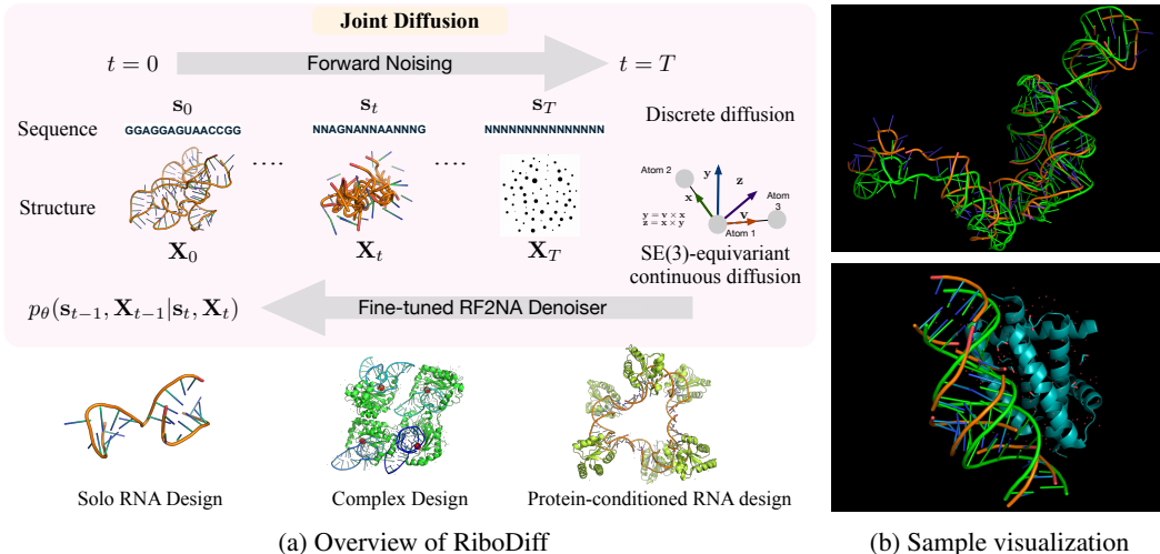
Figure 1: (a) Joint diffusion with pre-trained priors for RNA co-design. Starting from clean sequence–structure, the forward process applies discrete diffusion to nucleotides and SE(3) -equivariant diffusion to all-atom frames. We fine-tune the pre-trained RF2NA as the denoiser, enabling joint generation and flexible conditioning across multiple tasks. (b) Orange traces show co-designed RNAs while green traces are reference RNAs; cyan ribbons denote protein in conditional settings.
