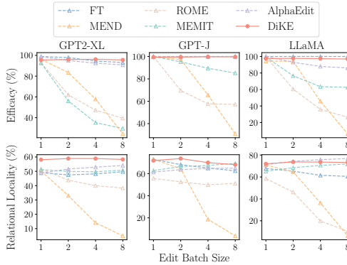
Figure 4: Performance of subject-consistent batch editing on the FINE-KED.
