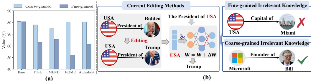
Figure 1: Knowledge editing can unintentionally affect fine-grained irrelevant knowledge. Figure (a): Preservation performance on fine-grained vs. coarse-grained irrelevant knowledge. Figure (b): Illustration of knowledge editing can unintentionally affect fine-grained irrelevant knowledge.
