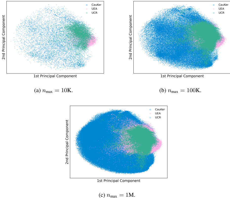
Figure 12: PCA-visualization of Mantis embeddings for samples from UCR, UEA and CauKer-generated data. For each plot, we randomly select \min(n_{\text{samples}}, n_{\text{max}}) samples for each dataset, where n_{\text{samples}} is the dataset size and n_{\text{max}} \in \{10\text{K}, 100\text{K}, 1\text{M}\} .
