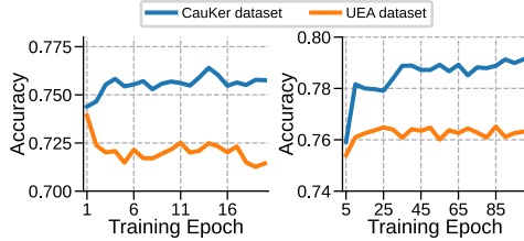
Figure 6: Test accuracy across epochs for MOMENT (left) and Mantis (right).
