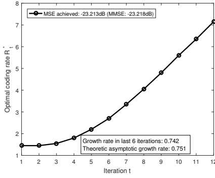
Fig. 1. Low-EMSE growth rate of optimal coding rate sequence per DP vs. asymptotic growth rate \frac{1}{2} \log_2 \left( \frac{1}{\bar{\theta}} \right) . (BG signal (11), \rho = 0.2 , \kappa = 1 , P = 100 , \sigma_W^2 = 0.01 , b = 0.782 .)
