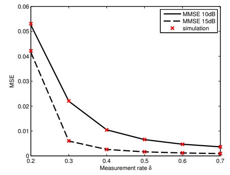
Fig. 3. Verification that C-MP-AMP achieves the MMSE at various measurement rates \kappa = M/N and SNR levels. ( P=3 , N=30000 .)
