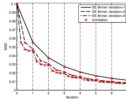
Fig. 2. Verification of SE for C-MP-AMP with various communication schedules. ( P=3 , N=30000 , M=9000 , \text{SNR}=15\text{dB} .)
