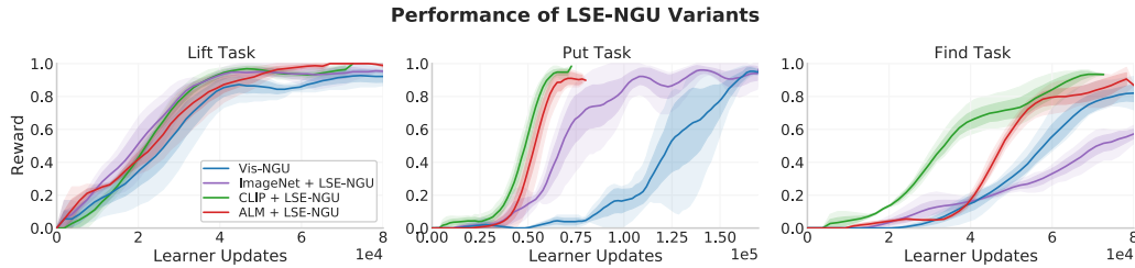
(b) LSE-NGU rewards novel pretrained image embeddings of O_V and does not use oracle language.
