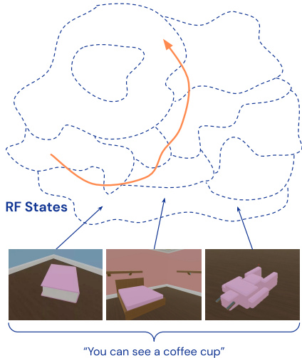
Figure 5: The dotted lines correspond to state abstractions given by the shuffled \hat{f}_S used in S-LD. The states are grouped together based on similarities in the visual random feature space and assigned a label. Exploring in this shuffled space is less effective than exploring with the semantically-meaningful abstractions shown in Figure 1.
