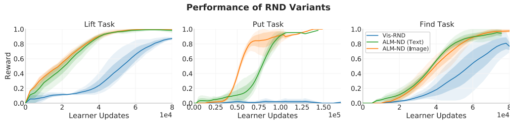
(c) ND intrinsic rewards derive from the prediction error of the representations from a pretrained ALM network.
