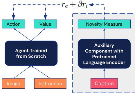
Figure 3: The agent is trained from scratch using RL to optimize extrinsic and intrinsic reward. It acts using the image observation O_V and goal g . During training, the novelty-based intrinsic reward is calculated using an auxiliary component that does not share parameters with the agent (dashed box). The auxiliary component may incorporate a pretrained language (pictured above) or image encoder, which may respectively require O_L or O_V . The latter does not rely on language provided by the environment. See Figure S2 for more details.
