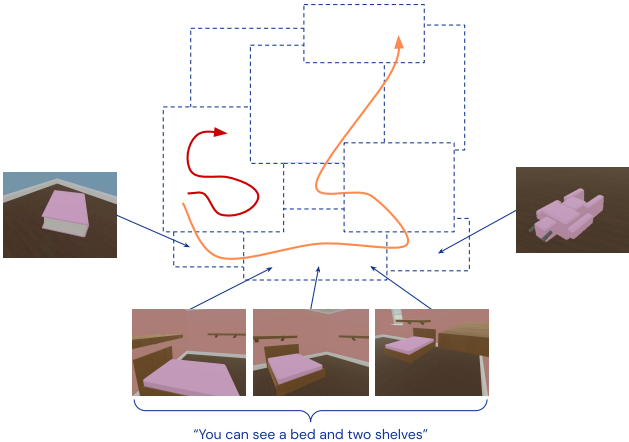
Figure 1: Navy dashed lines delineate semantically meaningful states. By using representations that align well with these boundaries (i.e. language), then agents more effectively explore the wider state space (orange trajectory). If the representations do not reflect these boundaries and instead are amenable to visual noise (i.e. different colors, viewpoints, etc.), then agents may only focus on a visually novel, yet narrow subset of states (red trajectory).
