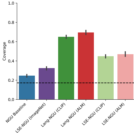
Figure 6: Coverage of City (number of bins reached on map) by NGU variants using different state representations for exploration, normalized by coverage of a ground-truth agent. The ground-truth agent represents state in NGU as the global coordinate of the agent location. The dashed line indicates coverage of a uniform random policy. Error bars indicate standard error of the mean, over 5 replicas. See Appendix Table S4 for absolute coverage numbers.
