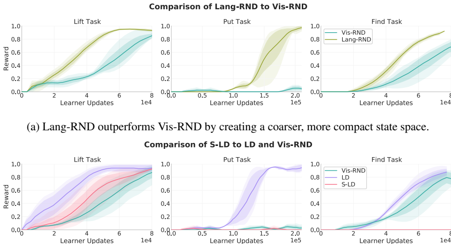
(b) LD outperforms S-LD. It is important how language abstractions carve up the state space.
