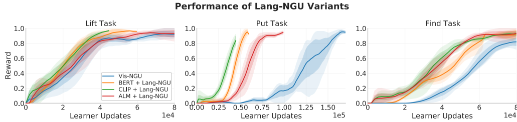
(a) Lang-NGU rewards novel pretrained text embeddings of O_L .
