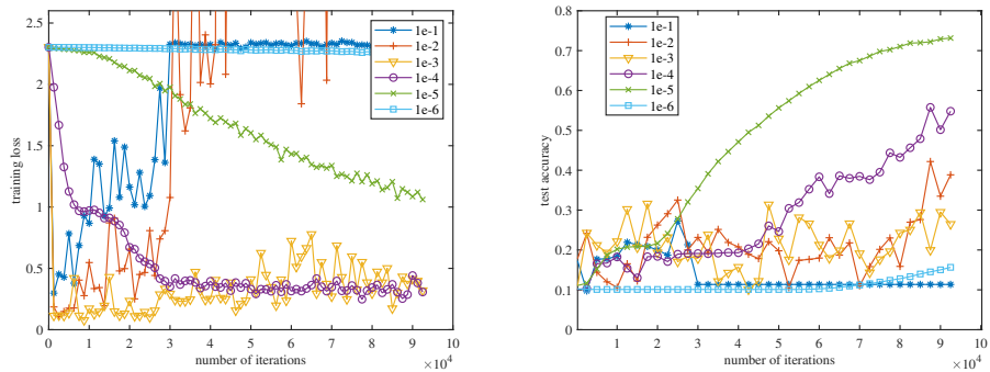
(a) Training loss (b) Test accuracy Figure 4: Performance comparison of different stepsizes for DADAM
