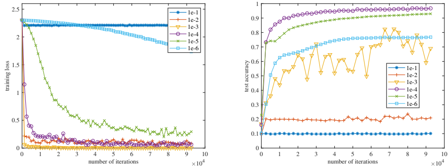
(a) Training loss (b) Test accuracy Figure 3: Performance comparison of different stepsizes for decentralized AMSGrad
