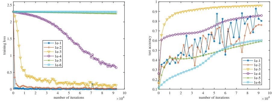
(a) Training loss (b) Test accuracy Figure 2: Performance comparison of different stepsizes for DGD
