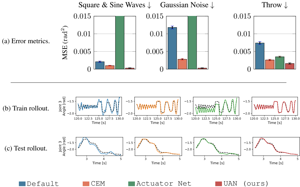
Figure 6: UAN achieves the tightest real-to-sim fit to the training data, as well as a throw trajectory unseen during training. We rolled out three real-world joint trajectories: square & sine waves at each joint, Gaussian noise across all the joints, and a throw. Square waves, sine waves, and gaussian noise were seen during training, while the throw was not. We found that Actuator-Net error remains bounded on the 5 s throw trajectory but diverges when rolling out the 5 min training trajectories, while the UAN learned to remain accurate across long rollouts through RL training.
