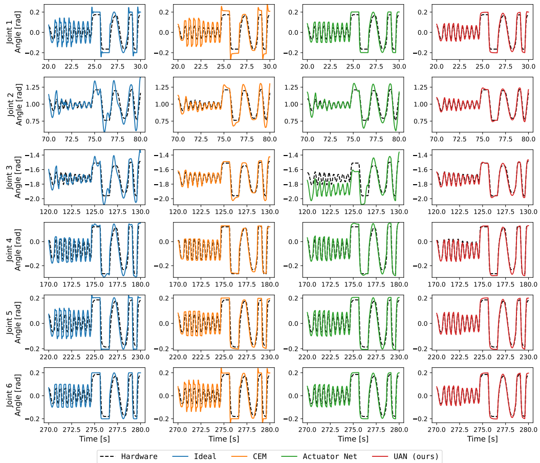
Figure 8: Comparison of system identification methods on open-loop rollouts of the training data.
