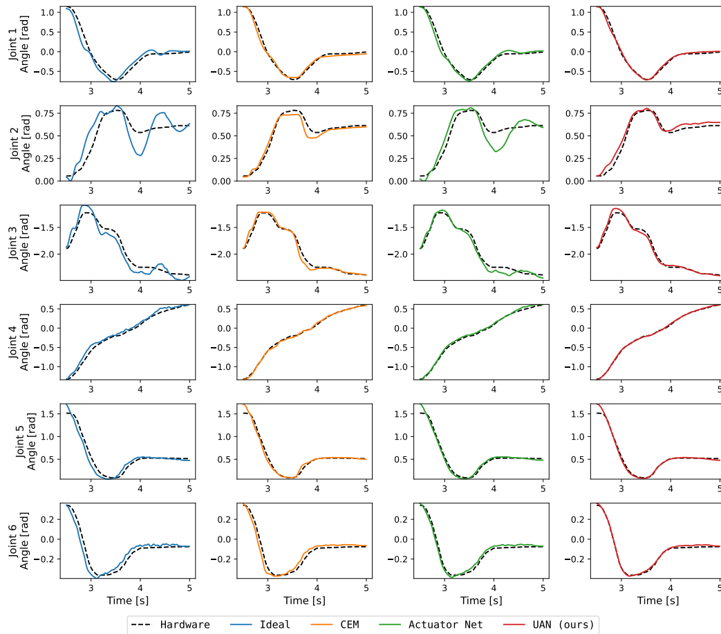
Figure 9: Sim-to-real gap for a throwing trajectory unseen during training.
