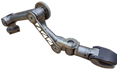
Figure 3: Unitree Z1 Pro arm. This arm’s harmonic actuators behave substantially differently from the quasi-direct-drive motors common in small legged robots. This image also shows the reinforcements we designed to ensure that the limit on athleticism comes from actuation rather than the linkage structural integrity.
