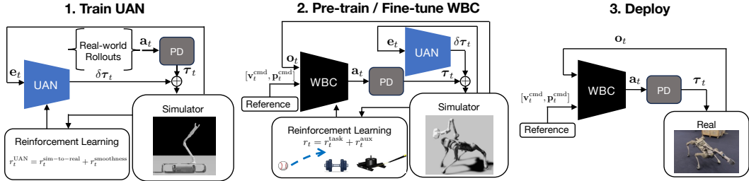
Figure 2: Unsupervised Actuator Network (UAN) approach for real-to-sim-to-real. Our training pipeline involves three steps: 1) Train a UAN to close the sim-to-real gap for actuators with complex transmission mechanisms by mapping a history of joint position and velocity errors, e_t , to corrective torques, \delta\tau_t , 2) Pre-train a WBC using random motion references (base velocity and EE pose), then and fine-tune it on an athletic task reward with the UAN in loop, and 3) Deploy. During the fine-tuning phase, the WBC initially tracks the task-specific reference, and then gradually learns to depart from the reference to maximize task performance.
