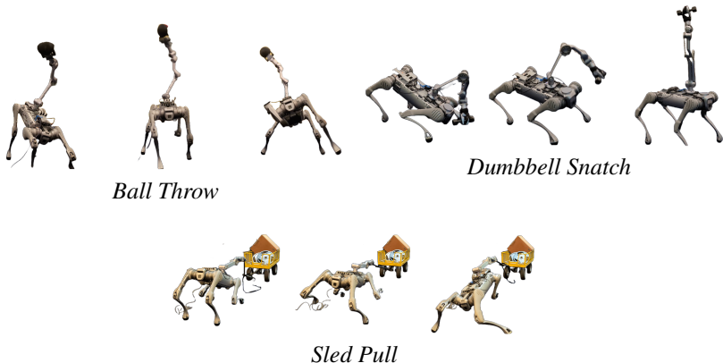
Figure 1: Sim-to-real transfer of athletic loco-manipulation. We reduce the sim-to-real gap for a quadruped manipulator by learning a corrective model for the simulated actuator dynamics based on real-world data , formulated as an unsupervised actuator net (UAN) . Policies trained with the corrected simulator exhibit improved sim-to-real transfer and push the limits of the robot’s physical capabilities in athletic tasks involving whole-body coordination. Videos of the robot’s behaviors are available at https://uan.csail.mit.edu/ .
