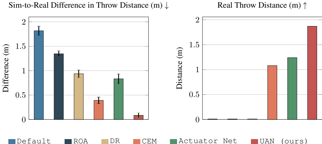
Figure 4: UAN improves simulator accuracy and real throwing performance. UAN (Ours) achieves lower sim-to-real difference in throw distance as compared to standard baselines, resulting in a better real throw distance. For this comparison, we train and test policies with a fixed-base arm, to avoid the risk of the legged base falling during performance-critical ablations.
