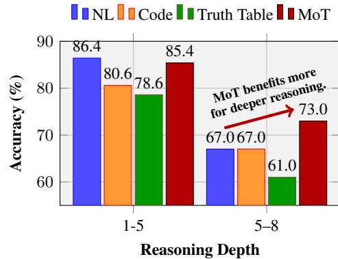
Figure 4: Performance comparison of different thought paradigms across reasoning depths. On FOLIO, MoT inference exhibits better performance on difficult problems.
