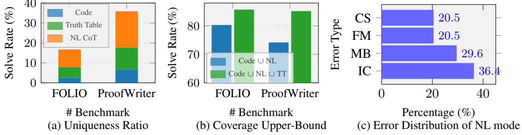
Figure 1: (a) Qwen-2.5-7B-Instruct solves \approx 20\% of FOLIO and \approx 35\% of ProofWriter exclusively per paradigm. (b) Code+NL+truth-table yields higher upper-bound coverage than code+NL alone [Xiong et al., 2024]. (c) In NL modes, invalid-converse (IC) and missing-branch (MB) errors comprise \approx 66\% of failures (CS: commonsense injection; FM: factual misquote). Percentages sum to more than 100% because some cases exhibit multiple error types. We provide illustrative examples in Appendix G.1
