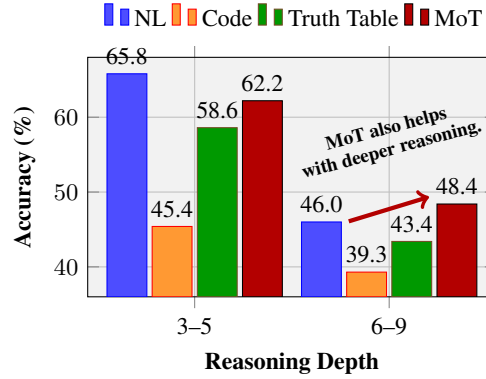
Figure 7: Performance comparison of different thought paradigms across reasoning depths. On ProverQA, MoT inference exhibits better performance on difficult problems.
