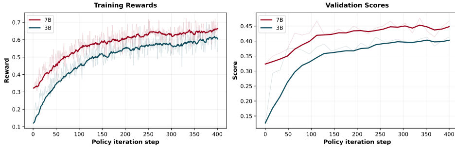
Figure 10: Learning curves of vision-language agents. We RL-tune Qwen2.5-VL-3B/7B-Instruct using Dr. GRPO on the math:Geometry3K environment and track their training rewards (left) and validation scores (right).
