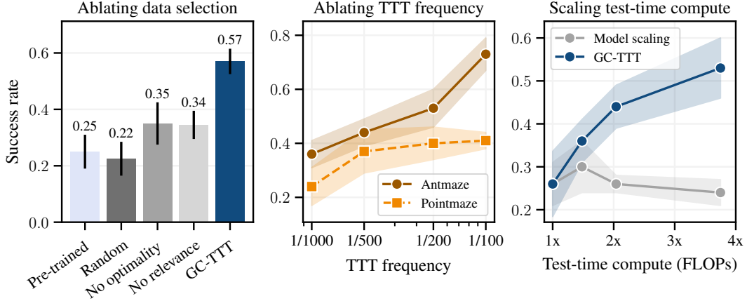
Figure 6: Left: Ablation of the data selection criteria. Both relevance and optimality have to be considered to filter the dataset for test-time training. Middle: Allocating more compute by increasing the frequency of TTT improves performance, and saturates slightly earlier in simpler environments. Right: We compare scaling test-time compute of GC-TTT (by increasing TTT frequency) to scaling the policy networks such that inference FLOPs are matched, within the antmaze play environment. We find that GC-TTT scales well with increased test-time compute, while scaling model size does not yield significant improvements.
