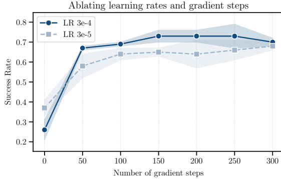
Figure 7: GC-TTT results for different gradient steps.
