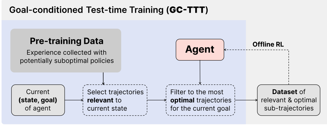
Figure 2: GC-TTT specializes the agent to the next steps for achieving its target goal.
