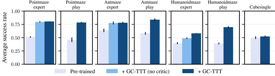
Figure 5: Success rates of GC-TTT within each environment, averaged across RL backbones.
