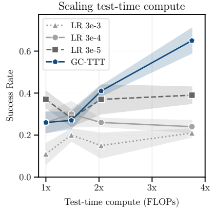
Figure 8: Model scaling results for different learning rates.
