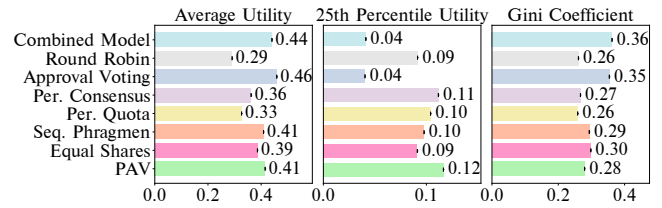
Figure 6: Performance of the different rules on the Moral Machine Dataset, based on high-disagreement alternatives, for T = 100 rounds with each round having 100 alternatives and each voter approving their top 1 alternative.
