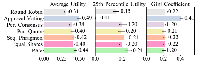
Figure 4: Performance of the rules on synthetic instances. The length of the bar shows the median across the 1000 trials, the error bars give the 25th and 75th percentile, and the numeric text gives the mean.
