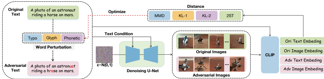
Figure 2: An illustration of our proposed attack method for evaluating the robustness of T2I DMs.
