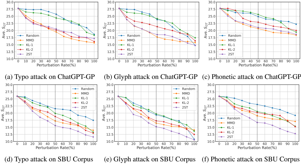
Figure 3: CLIP Score at different perturbation rates on ChatGPT-GP and SBU Corpus.
