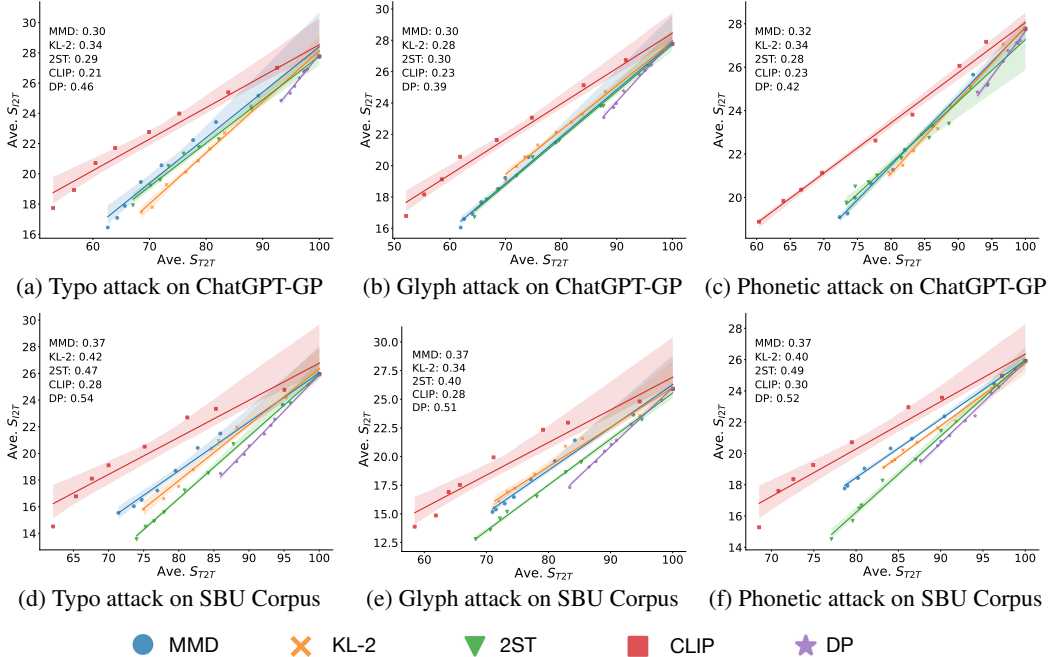
Figure 4: Correlation between S_{I2T} and S_{T2T} on ChatGPT-GP and SBU Corpus. The numbers in the upper-left corner represent the slopes of the plotted lines.
