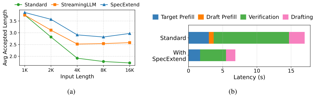
Figure 4: (a) Average accepted length of Vicuna-7B/68M across different draft model cache settings. (b) End-to-end latency breakdown of speculative decoding on 16K-token inputs.
