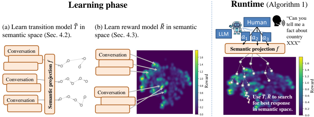
Figure 1: Overview of our approach, SCOPE, that automatically learns the reward associated with each LLM response for conversation planning. During learning phase (left), we exploit dense semantic representation of conversations to learn a lightweight transition and reward model in semantic space (Notations and details covered in Sections 4.2 and 4.3). During runtime (right), SCOPE uses these learnt models to perform MCTS in semantic space without needing additional LLM queries for simulation (Algorithm 1), allowing us to find the optimal LLM response that maximizes the cumulative reward in a conversation.
