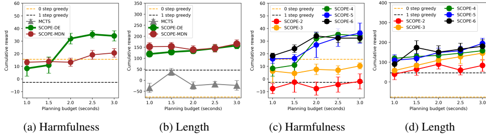
Figure 11: (a) and (b): Ablation study on how transition model choice affects SCOPE’s performance. SCOPE-DE uses deep ensembles (Lepikhin et al., 2021) while SCOPE-MDN uses MDNs (Bishop, 1994). (c) and (d): Ablation study on how search depth affect SCOPE’s performance.
