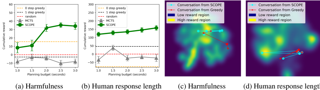
Figure 3: (a) and (b) show the average cumulative rewards (higher is better) gathered by SCOPE compared to other baselines over 100 different conversation starters for the harmfulness and human response length reward function over 5 conversation turns. The x -axis shows the effect of increased planning budget (time). (c) and (d) show visualization of a conversation generated from SCOPE and 1-step Greedy in the semantic space.
