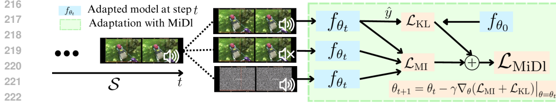
Figure 2: Adapting at test-time with MiDI. At test time, the stream reveals a sample. MiDI uses multimodal samples to adapt and requires one forward pass for each modality combination. MiDI leverages (KL) divergence to align the predictions of the adapted model f_{\theta_t} with those of the original model f_{\theta_0} , ensuring that the adapted model does not deviate too far from the original model’s predictions. The Mutual-Information (MI) component uses the prediction from the different modalities to reduce the dependency on any specific modality, fostering a more generalized and robust prediction across different modality combinations. MiDI updates the model for step t + 1 using the combination of KL and MI in Equation 2.
