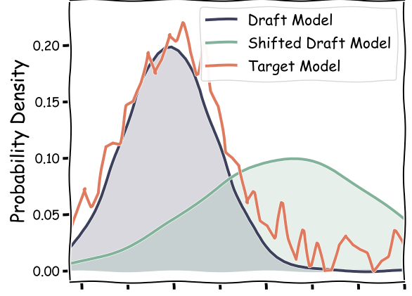
Figure 1: Shifted draft model reflects human preferences, but presents a gap from unaligned target model.
