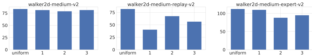
Figure 6: Normalized average performance of the proposed method (uniform on the X-axis) and latent policies with clipped normal latent distribution. Number on the X-axis is the clipping value. Optimal clipping value is different for each dataset and final performance is better for the proposed method.
