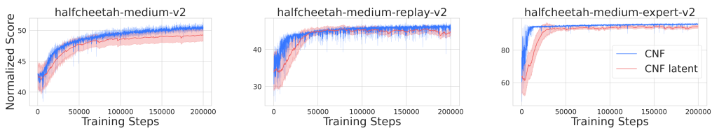
Figure 9: Comparison of CNF trained in original (blue) and latent (red) action spaces. Final performance is slightly lower for the training directly in latent space.
