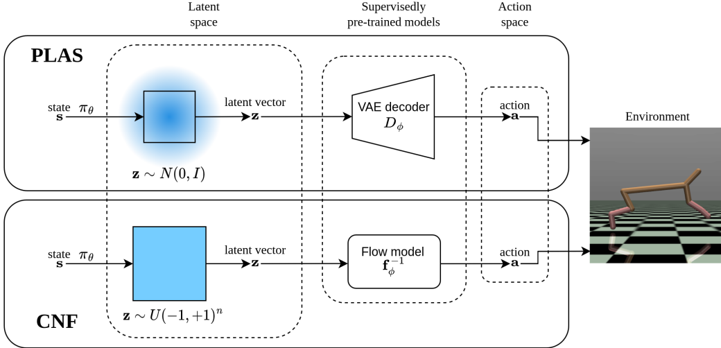
Figure 1: Schematic visualization and comparison of PLAS and CNF (ours) approaches. Both methods use an action encoder-decoder model trained in a supervised manner on an offline dataset and a controller model to select actions from the latent space of the encoder. PLAS algorithm uses VAE with normal latent distribution with unbounded support (represented as the blue circle) and restricts latent policy outputs to only a part of the latent space (represented as the black borders inside of latent space). Our algorithm uses Normalizing Flow instead of VAE and bound base distribution itself, allowing the latent policy to use the whole latent space.
