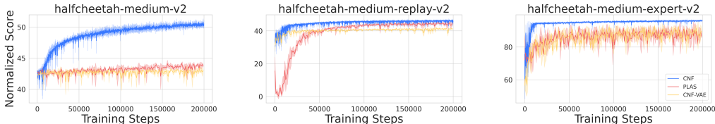
Figure 7: Comparison of CNF, CNF with VAE (CNF-VAE) and PLAS. CNF with Normalizing Flow and uniform distribution performs above all. For normal distribution optimal clipping value is different for each dataset.
