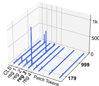
Figure 30: DINOv2-reg ViT-G.
