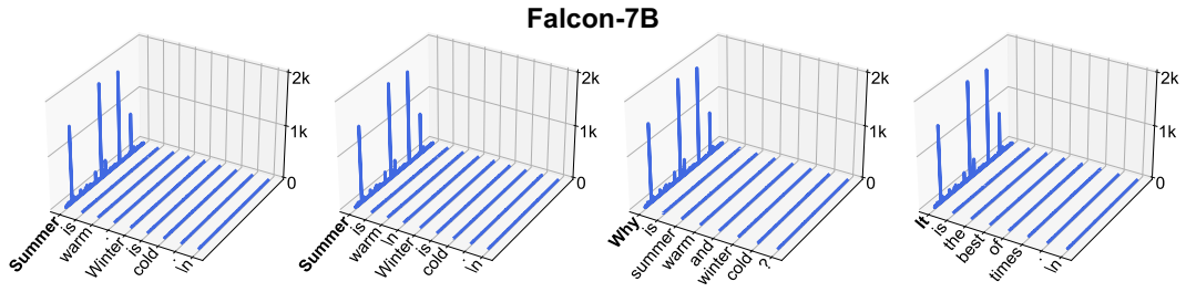
Figure 12: Massive activations in Falcon-7B.
