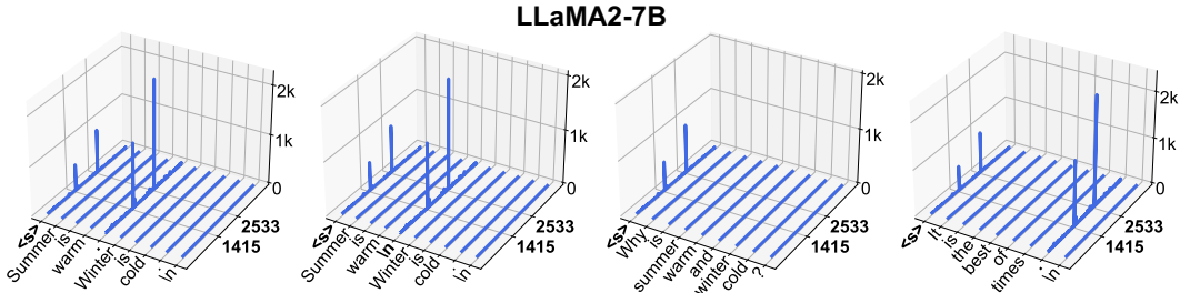
Figure 17: Massive activations in LLaMA2-7B when the input is prepended with a BOS token \langle s \rangle .
