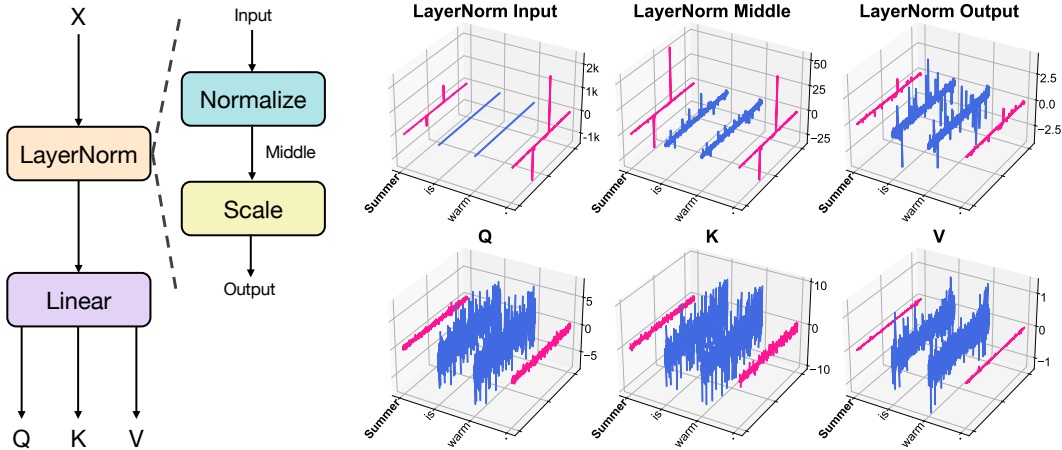
(a) Attention LayerNorm and QKV linear projections. (b) Layer 3, LLaMA2-7B. We highlight the embeddings of the two tokens where massive activations appear: the starting token and the period token.
