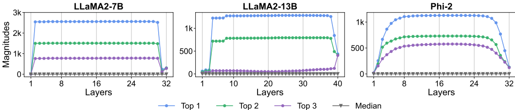
Figure 2: Three largest activation magnitudes and the median magnitude at each layer in LLMs.
