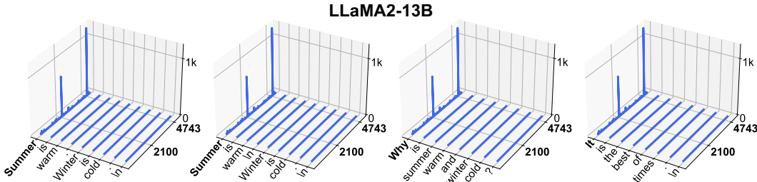
Figure 6: Massive activations in LLaMA2-13B. In this model, they appear in two fixed feature dimensions (2100, 4743), and are limited to the starting token.
