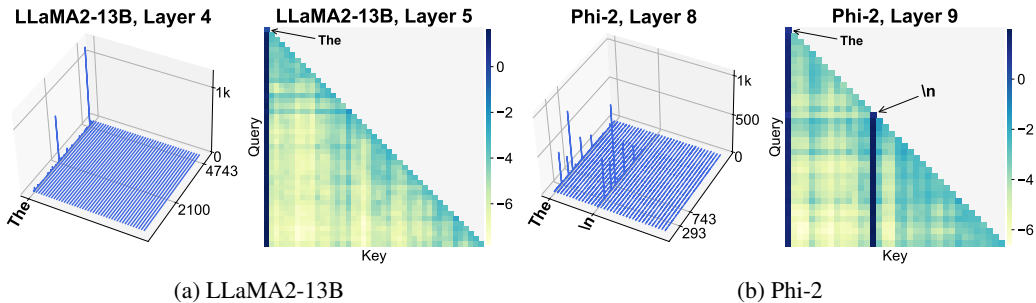
Figure 21: Attention patterns after massive activations emerge in LLaMA2-13B and Phi-2.
