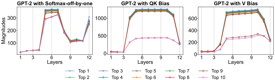
Figure 26: Ten largest activation magnitudes at each layer in three GPT-2 models.
