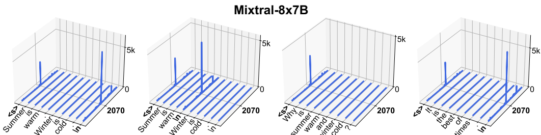
Figure 19: Massive activations in Mixtral-8x7B when the input sequence is prepended with a BOS token \langle s \rangle .
