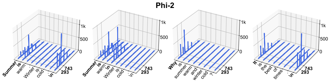
Figure 9: Massive activations in Phi-2.
