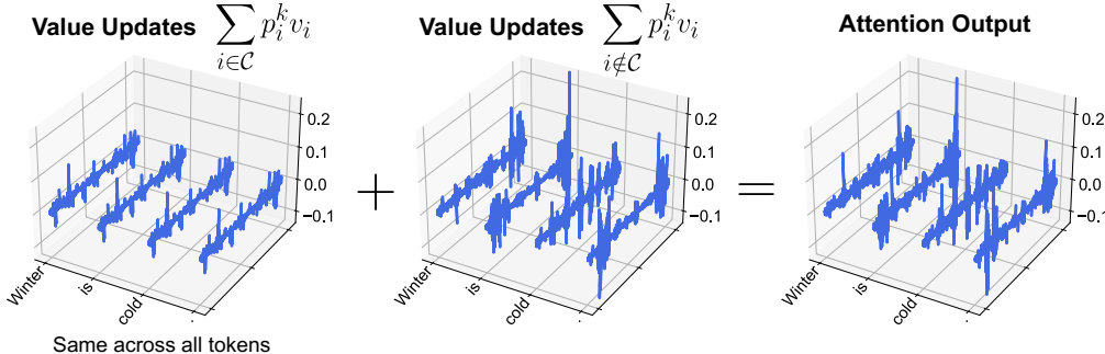
Figure 5: Value updates from tokens associated with massive activations are essentially the same.
