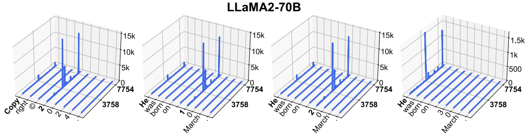
Figure 8: Massive activations in LLaMA2-70B.
