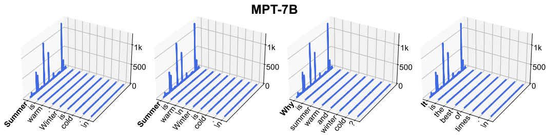
Figure 11: Massive activations in MPT-7B.
