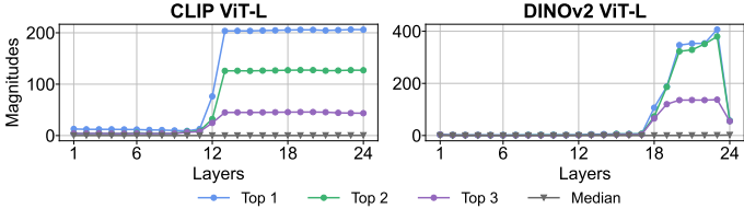
Figure 29: Three largest activation magnitudes and the median magnitude at each layer in CLIP and DINOv2 ViT-L.
