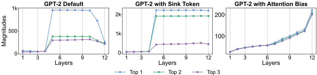
Figure 25: Three largest activation magnitudes in the output feature of each layer for three GPT-2 models.
