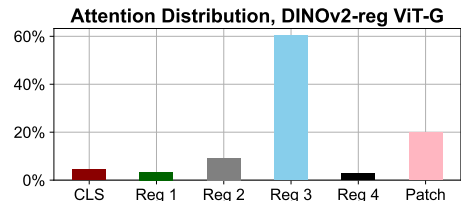
Figure 32: Average attention of the [CLS] token.
