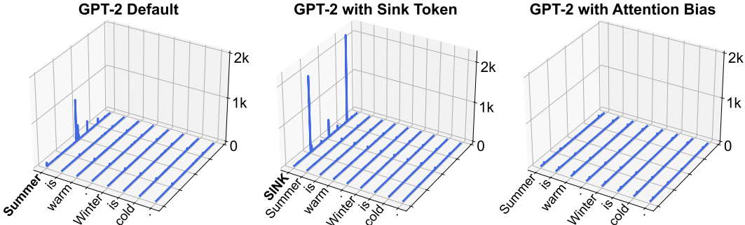
Figure 24: Massive activations disappear when training GPT-2 with explicit attention bias (Equation 3).
