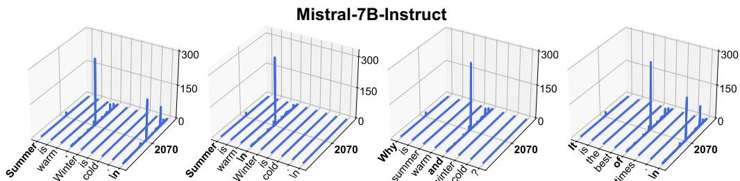
Figure 15: Massive activations in Mistral-7B-Instruct.
