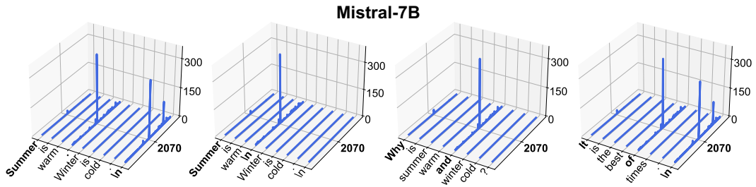
Figure 10: Massive activations in Mistral-7B.
