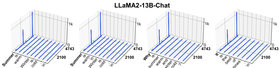
Figure 14: Massive activations in LLaMA2-13B-Chat.
