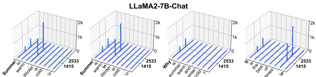
Figure 13: Massive activations in LLaMA2-7B-Chat.
