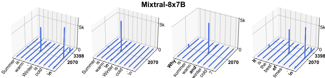
Figure 7: Massive activations in Mixtral-8x7B. In this model, they lie in two feature dimensions (2070, 3398), and are found within the starting token, delimiter tokens and certain word tokens (“and” and “of”).
