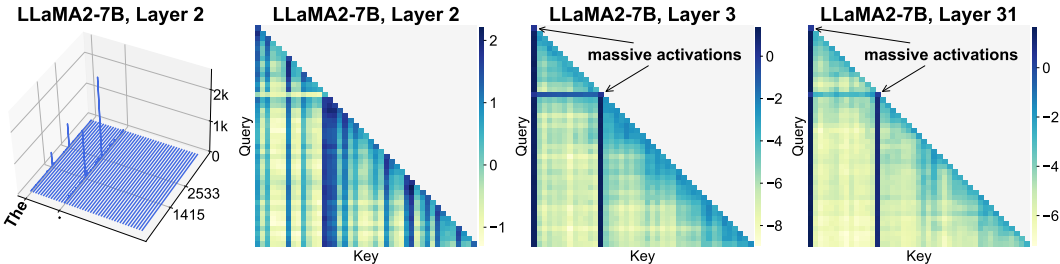
Figure 3: Attention patterns before and after massive activations appear in LLaMA2-7B. For each layer, we visualize average attention logits over all heads, for an input sequence.
