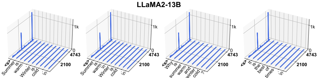
Figure 18: Massive activations in LLaMA2-13B when the input sequence is prepended with a BOS token \langle s \rangle .
