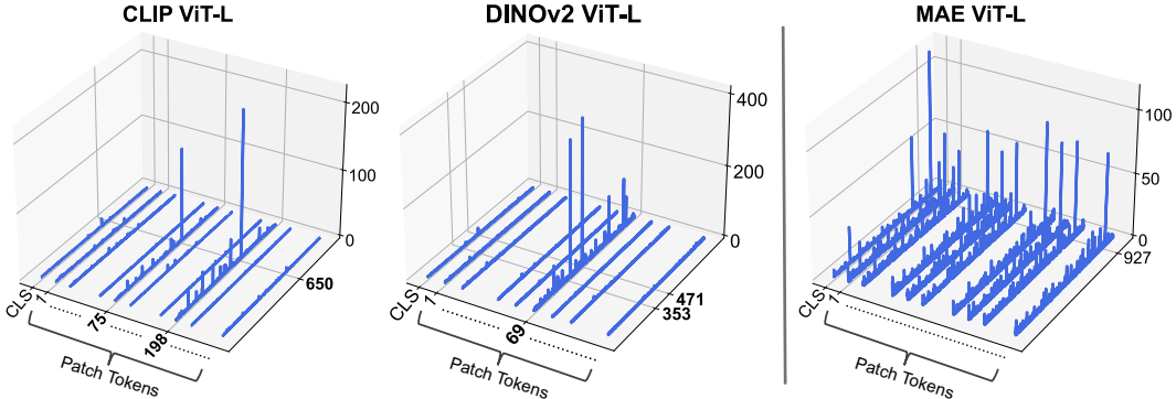
Figure 27: Massive activations are present in ViT-L from CLIP and DINOv2, but not MAE.
