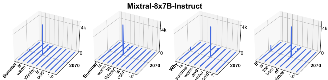
Figure 16: Massive activations in Mixtral-8x7B-Instruct.
