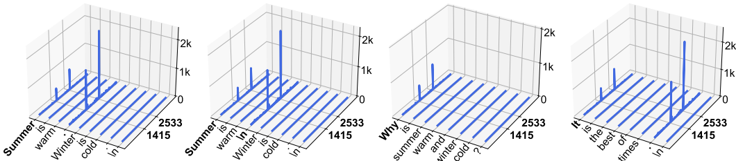
Figure 1: Activation Magnitudes (z-axis) in LLaMA2-7B. x and y axes are sequence and feature dimensions. For this specific model, we find that activations with massive magnitudes appear in two fixed feature dimensions (1415, 2533), and two types of tokens—the starting token, and the first period (.) or newline token (\n).
