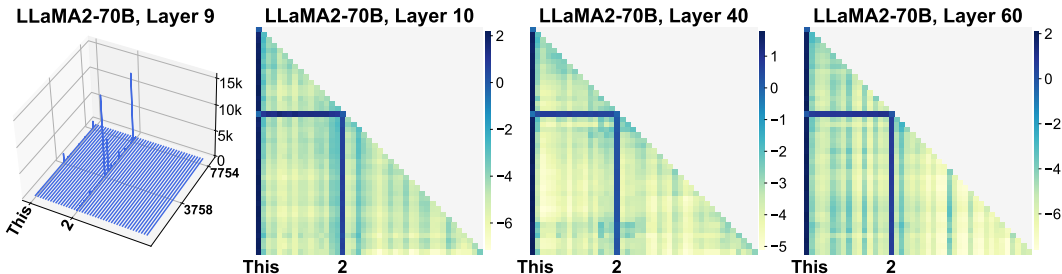
Figure 22: Average attention logits over all heads in layers 10, 40 and 60 of LLaMA2-70B. The input sequence is “This book, including all illustrations and text, is protected under Copyright©2024 and may not be reproduced or transmitted in any form without the prior written permission of the copyright owner.”.
