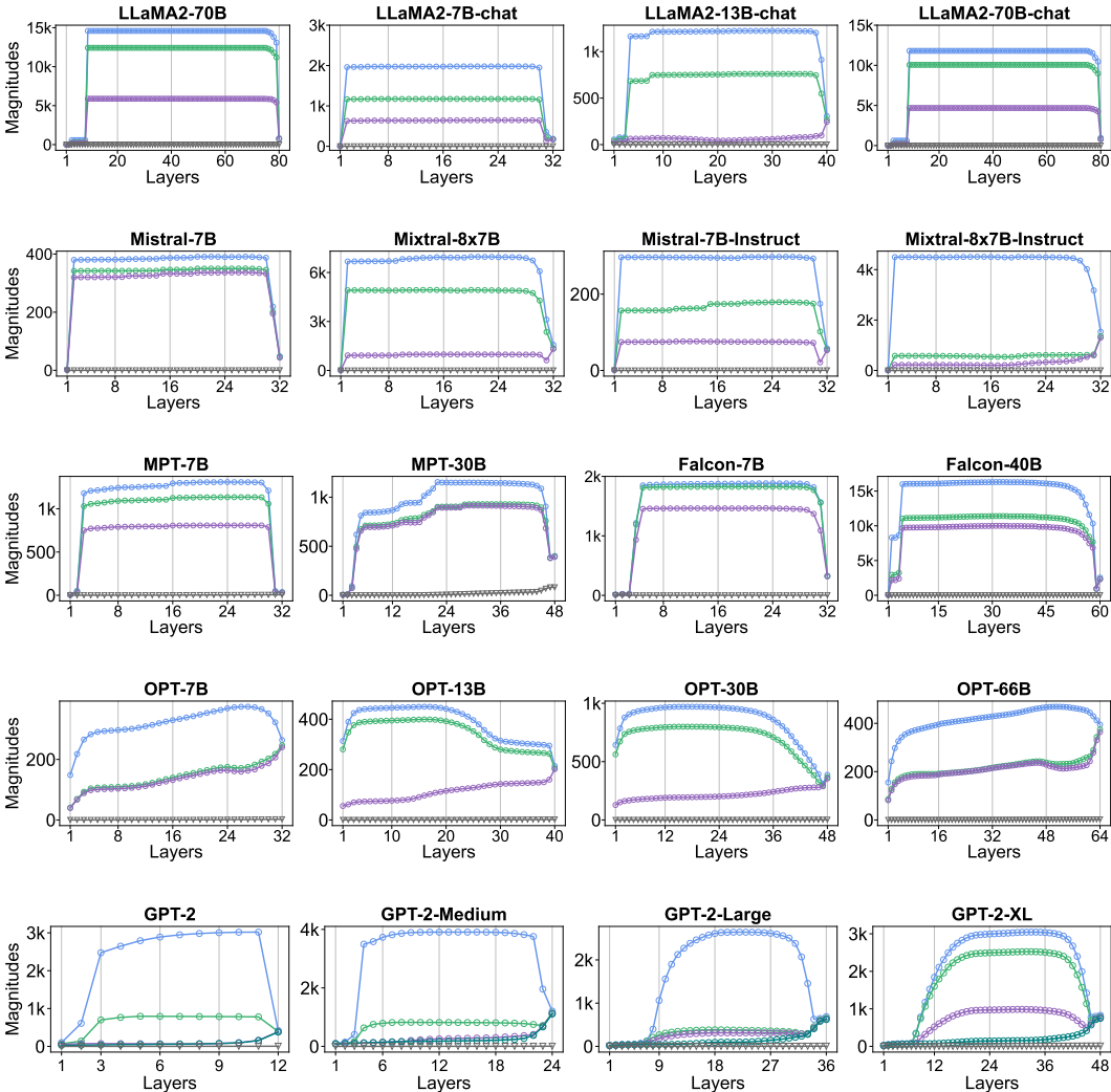
Figure 20: Layer-level analysis of LLMs. For each model, we show the three largest activation magnitudes as well as the median per layer.
