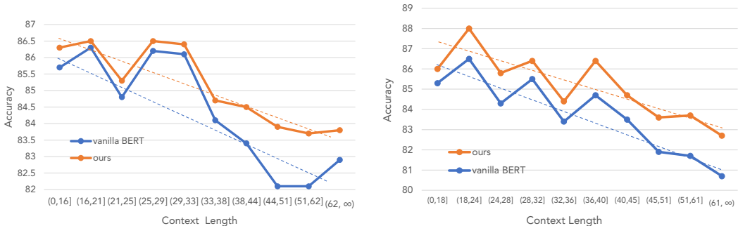
Figure 4: Accuracy of different context length on MNLi-match (left) and MNLi-mismatch (right) dev set. There are approximate 1000 samples in each intervals.
