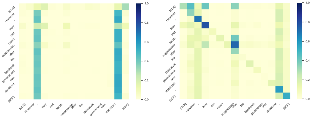
Figure 3: Heatmap of the attention matrix of vanilla BERT and our implemented PROPHET for the sentence "However, they met harsh suppression after the Bolthevik government was stabilized.". Weights are selected from the first head of the last attention layer.
