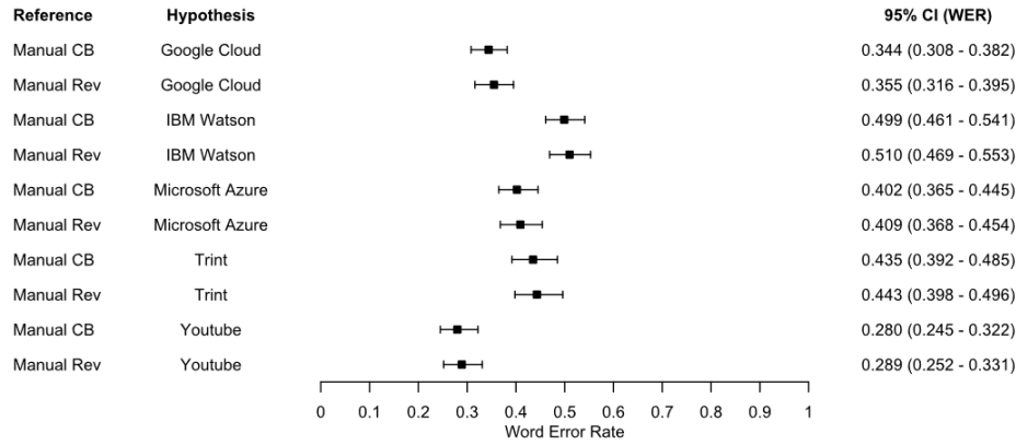
Fig. 1. Forest plot of WER of automatic transcription services, using two sets of reference transcripts from each of the two manual transcription services (Manual CB and Manual Rev).
