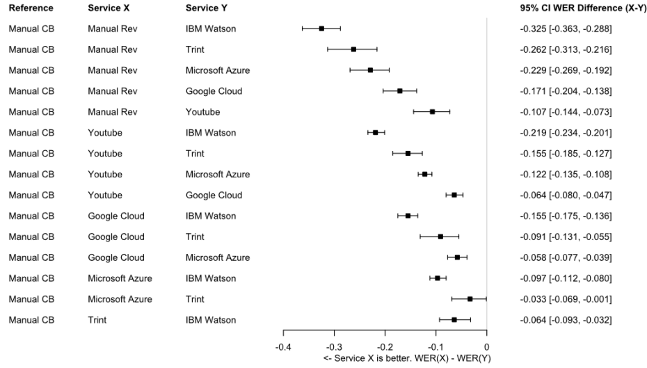
Fig. 2. Forest plot of pair-wise differences in WER of the various transcription services. Only comparisons where Service X is better are illustrated. The plot is ordered by the best performing service in Service X, followed by the mean WER difference between Service X and Service Y.
