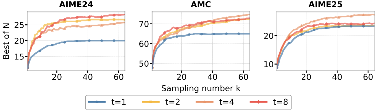
Figure 11. BoN (Best-of-N) decoding on the AIME2024, AMC, and AIME2025 benchmarks using Temporal Sampling. Qwen2.5-Math-PRM-72B is used as the process reward model. We choose the answer with the highest reward as the final answer. The case t = 1 represents the baseline of standard BoN on the final checkpoint. Our proposed Temporal Sampling with t = 8 checkpoints outperforms the baseline by more than 7, 8, and 1 percentage points on AIME2024, AMC, and AIME2025, respectively, when sampling 64 responses.
