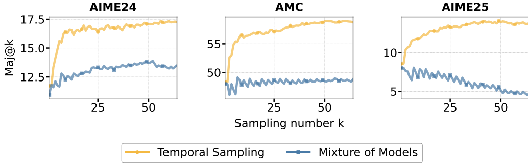
Figure 9. Maj@ k comparison between Temporal Sampling ( t = 3 ) and a Mixture of Models (MoM) approach on the AIME2024, AMC, and AIME2025 benchmarks. For MoM, the model pool included the Qwen2.5-7B-Base final RL checkpoint, Deepseek-Math-7B-Instruct, and Llama-3.1-8B-Instruct. Temporal Sampling outperforms the MoM approach by more than 4, 9, and 9 percentage points on AIME2024, AMC, and AIME2025, respectively, when sampling 64 responses.
