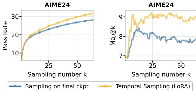
Figure 10. Performance of Temporal Sampling using 8 checkpoints from LoRA SFT of Qwen2.5-7B. Results on the AIME demonstrate that Temporal Sampling with LoRA checkpoints surpasses the baseline (sampling only from the final checkpoint) for both Pass@k and Maj@k .
