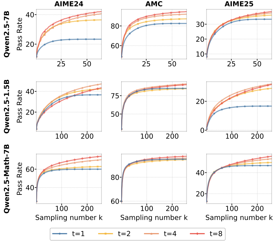
Figure 6. Pass@k for different numbers of checkpoints t on the AIME2024, AMC, and AIME2025 benchmarks when using Temporal Sampling. The case t = 1 represents the baseline of standard Pass@k sampling on the final checkpoint. Our proposed Temporal Sampling for Qwen2.5-7B with t = 8 outperforms the baseline by more than 19, 13, and 4 percentage points on AIME2024, AMC, and AIME2025, respectively, when sampling 64 responses.
