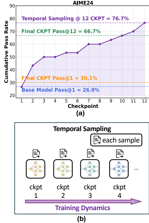
Figure 1. (a) We observed that during RL training process of Deepseek-R1-1.5B model, 76.7% of AIME problems were solved correctly at least once by some intermediate checkpoint, yet only 30% remained correct in the final model. This indicates that many problems answered correctly during training were ultimately incorrect in the final checkpoint. We term this phenomenon as Temporal Forgetting . (b) We proposed Temporal Sampling : This method utilizes training dynamics as a source of answer diversity by distributing inference samples across multiple distinct checkpoints from the training trajectory, rather than relying solely on the single final checkpoint.
