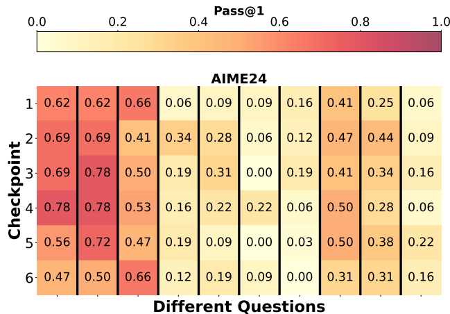
Figure 5. Pass rate distribution across training checkpoints on AIME24. Individual problems show varying pass rates over time. Temporal Sampling exploits these dynamics to improve answer diversity at inference.
