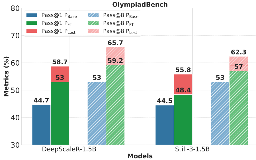
Figure 13. Performance of the base model ( P_{Base} ↑), the fine-tuned model ( P_{FT} ↑) and the Lost Score ( P_{Lost} ↓) for Pass@1 sampling and Pass@8 sampling. Fine-tuned models like DeepScaleR-1.5B (Luo et al., 2025) and Still-3-1.5B (Face, 2025) outperform the base model overall but also forget many questions the base model answered correctly.
