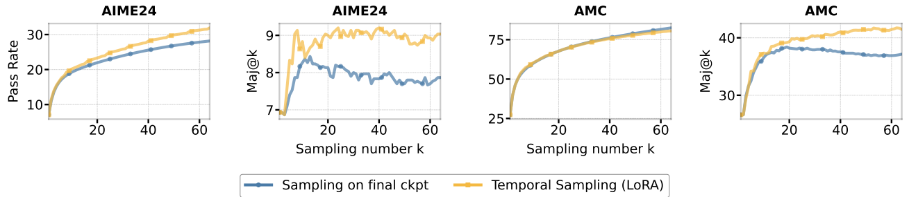
Figure 14. Performance of Temporal Sampling using 8 checkpoints from LoRA SFT of Qwen2.5-7B. Results on the AIME24 and AMC demonstrate that Temporal Sampling with LoRA checkpoints surpasses the baseline (sampling only from the final checkpoint) for both Pass@k and Maj@k .
