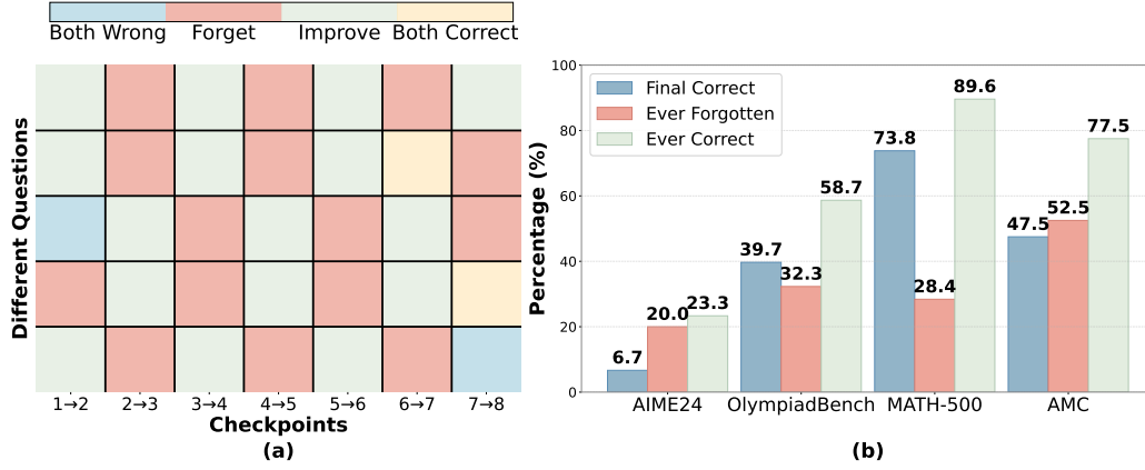
Figure 4. Forgetting dynamics of Qwen2.5-7B during RL training. (a) Answer correctness trajectories for OlympiadBench questions across training checkpoints, illustrating solutions oscillate between correct and incorrect states. "Forget" implies that an answer was correct at the previous checkpoint but incorrect at the current one. Conversely, "Improve" implies that an answer that was incorrect at the previous checkpoint but correct at the current one. (b) Percentage of questions per benchmark that are ever forgotten or ever correct at some checkpoint during GRPO.
