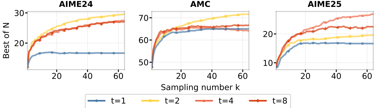
Figure 12. BoN (Best-of-N) decoding on the AIME2024, AMC, and AIME2025 benchmarks using Temporal Sampling. Qwen2.5-Math-PRM-7B is used as the process reward model. We choose the answer with the highest reward as the final answer. The case t = 1 represents the baseline of standard BoN on the final checkpoint. Our proposed Temporal Sampling with t = 8 checkpoints outperforms the baseline by more than 10, 2, and 5 percentage points on AIME2024, AMC, and AIME2025, respectively, when sampling 64 responses.
