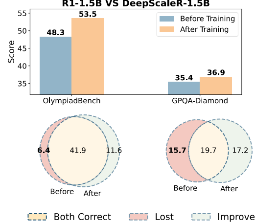
Figure 2. Overall performance score cannot tell everything. Fine-tuned models like DeepScaleR-1.5B (Luo et al., 2025) outperform the base model, R1-1.5B (DeepSeek-AI, 2025), overall but also forget many questions the base model answered correctly.
