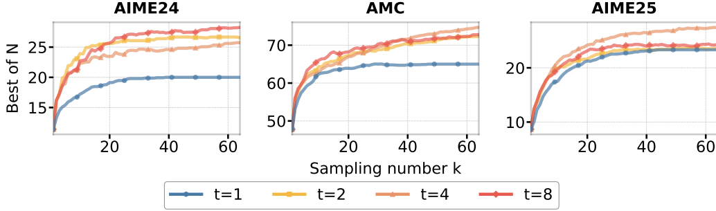
Figure 8. Best-of-N decoding on the AIME2024, AMC, and AIME2025 benchmarks using Temporal Sampling. The case t = 1 represents the baseline of standard BoN sampling on the final checkpoint. Our proposed Temporal Sampling with t = 8 checkpoints outperforms the baseline by more than 7, 8, and 1 percentage points on AIME2024, AMC, and AIME2025, respectively, when sampling 64 responses.
