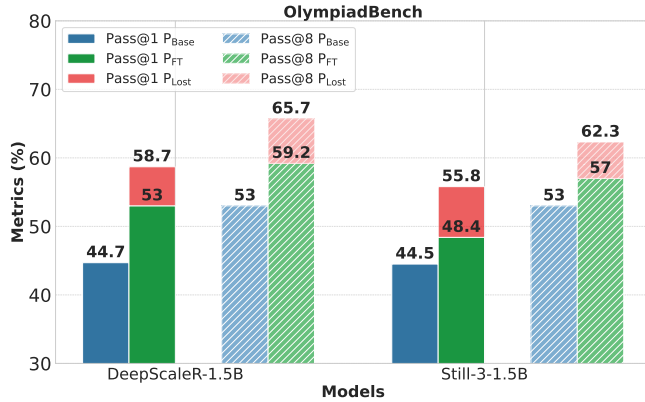
Figure 3. Performance of base model ( P_{Base} \uparrow ), fine-tuned model ( P_{FT} \uparrow ) and Lost Score ( P_{Lost} \downarrow ) for Pass@1 sampling and Pass@8 sampling. Models like DeepScaleR-1.5B (Luo et al., 2025) and Still-3-1.5B (Face, 2025) outperform the base model overall but also forget many questions the base model answered correctly when using diverse sampling.
