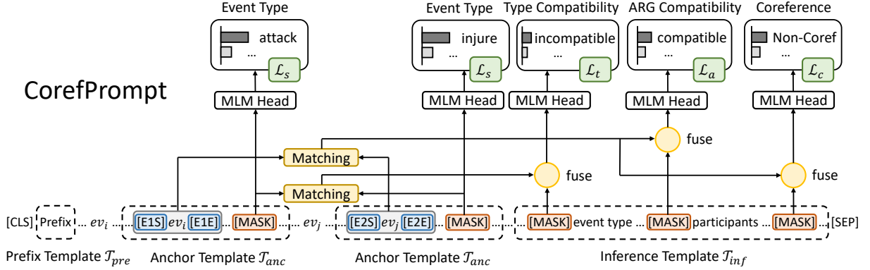
Figure 1: The overall framework of our prompt-based method CorefPrompt. We first utilize a prefix template \mathcal{T}_{pre} to inform PTM what to focus on when encoding, then mark event types and arguments by inserting anchor templates \mathcal{T}_{anc} around event mentions, and finally demonstrate the reasoning process of ECR using an inference template \mathcal{T}_{inf} which introduces two auxiliary prompt tasks, event-type compatibility and argument compatibility.
