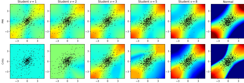
Figure 8: Qualitative comparison between ground-truth pointwise MI and learned critic for bivariate Student and normal distributions.
