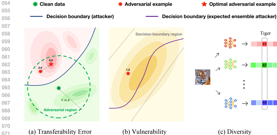
072 073 Figure 1: Vulnerability-diversity decomposition of transferability error. (a) The transferability error of 074 a given adversarial example is defined as the difference in expected loss value between that example 075 and the most transferable one. (b) Vulnerability is the loss value of the expected ensemble classifier 076 on the adversarial example. (c) Diversity represents the variance in model ensemble predictions that 077 correspond to the correct class.
