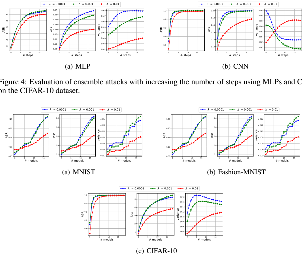
Figure 5: Evaluation of ensemble attacks with increasing the number of models using MLPs and CNNs on the three datasets.
