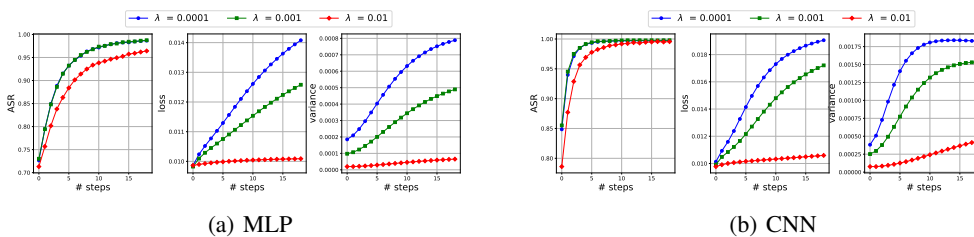
Figure 6: Evaluation of ensemble attacks with increasing the number of steps using MLPs and CNNs on the CIFAR-100 dataset.
