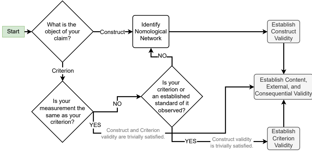
Figure 2: Decision process for establishing validity. For the decision processes that do not directly go through establishing construct or criterion validity, our argument is not that those forms of validity are irrelevant, but rather that they may be trivially satisfied in the context of the measurement, evaluation, and claim.
