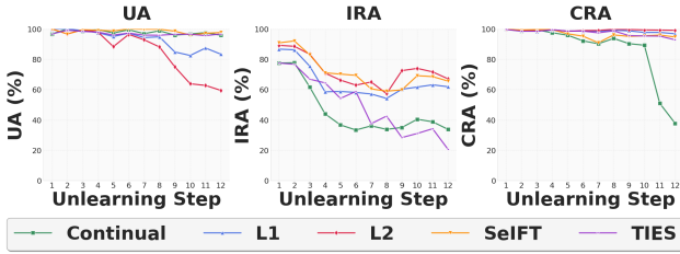
Figure 5. CA Object Unlearning, all proposed baselines outperform Continual in IRA and CRA, though L1 and L2 overwrites previous unlearning under long sequences. In this setting, SelfT achieves the best tradeoff between unlearning and retention. binary mask.
