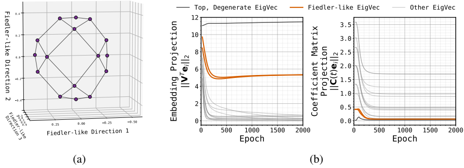
Figure 25: Spectral bias emergence in Node2Vec for grid graphs. (a) The Fiedler vectors of a grid graph capture spatial locality and connectivity patterns, closely mirroring the Node2Vec embedding shown in Figure 1 (bottom-right), where a similar geometry emerges. (b) Training dynamics show the same two-fold convergence pattern as path-star graphs, with embedding-Fiedler alignment and Fiedler vectors entering the co-efficient matrix null space.
