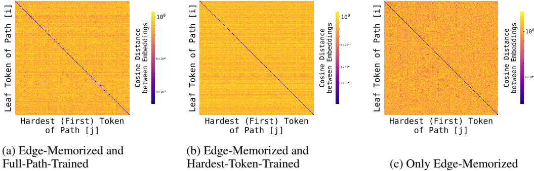
Figure 8: Evidence of global geometry in path-star task for Mamba . This figure is a counterpart to Figures 3 and 15 for the Mamba SSM architecture. Recall that entry (i, j) is the mean cosine distance between the leaf token in (an unseen) path i (row) and first/hardest token on (an unseen) path j (col). Each heatmap corresponds to a different training objective: Left: trained on edges and path-finding task ( \mathcal{D}_{\text{edge}} \cup \mathcal{D}_{\text{path}}^{\rightarrow} ); Middle: trained on edges and hardest-token-finding task (not presented in the main paper); Right: edges only ( \mathcal{D}_{\text{edge}} ). We find that even on these unseen paths, the leaf and first token embeddings cluster together, regardless of whether path-finding supervision exists. Interestingly, compared to the Transformer in Figure 15, the Mamba trained only on local supervision (right) exhibits a much stronger geometry.
