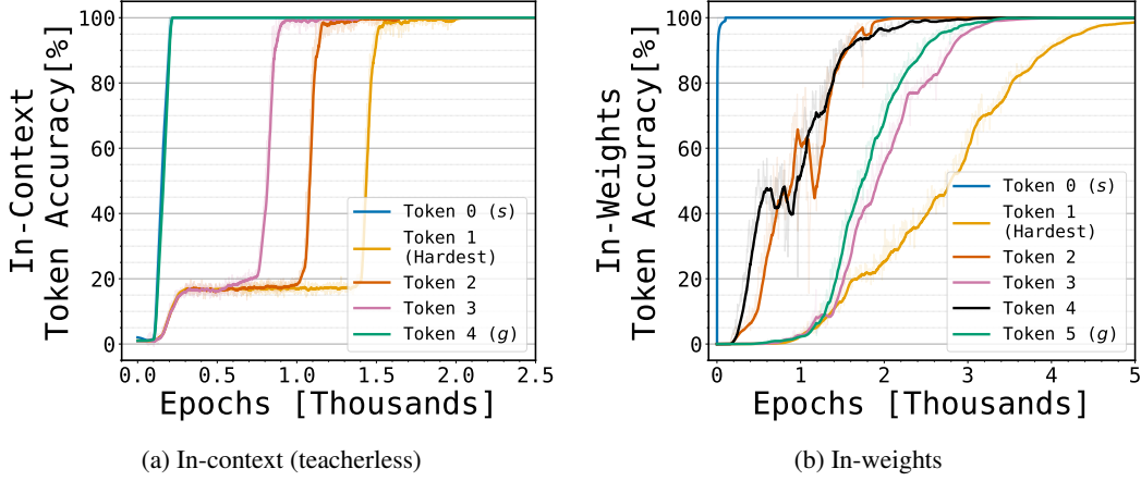
Figure 23: Learning dynamics per token. (a) In the in-context setting of \mathcal{G}_{2,5} (trained with a multi-token, teacherless objective since standard next-token prediction fails), later tokens are learned first indicating strong reliance on future-token signals. (b) In the in-weights setting of \mathcal{G}_{10^4,6} with next-token prediction, token accuracies rise largely in tandem (or in a somewhat confusing order); the first token is not selectively driven by future targets.
