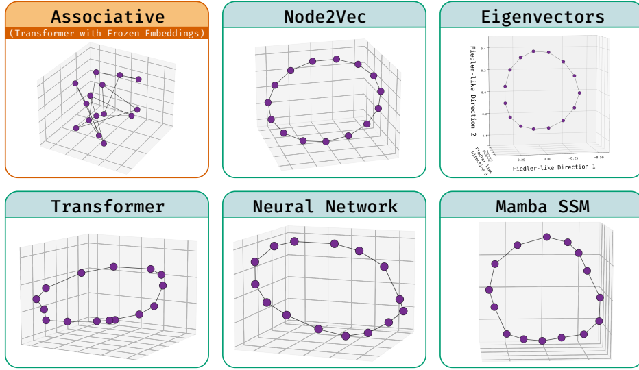
Figure 13: Tiny cycle : Geometries of various architectures on a small cycle graph. See Observation 4.
