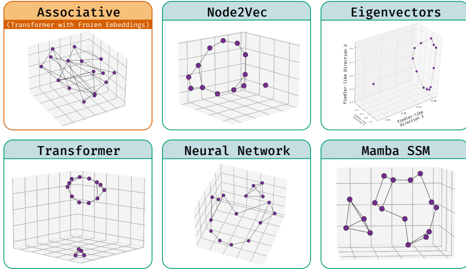
Figure 14: Tiny irregular graph : Geometries of various architectures on a small irregular graph of two connected components, both asymmetric. See Observation 4. Note that unlike in the other graphs, we do not use a 1-layer model here, but a 3-layered one.
