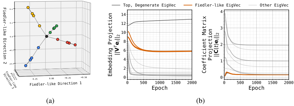
Figure 24: Spectral geometry arises in Node2Vec even without low-rank pressure (Observation 6) for Path-Star Graph. (a) The graph’s Fiedler vectors shown here closely mirrors the UMAP directions of the Node2Vec embeddings in Figure 1 (right). (b) The evolution of eigenvector projections during training. ( left ) The embedding matrix \mathbf{V} aligns with the Fiedler-like eigenvectors (and a top, degenerate vector) evidenced by the projection norm \|\mathbf{V}^T \mathbf{e}_i\|_2 converging to a stable, non-zero value. Projections of other eigenvectors diminish towards zero. ( right ) Concurrently, the Fiedler-like eigenvectors move into the null space of the co-efficient matrix \mathbf{C} in that the norm \|\mathbf{C} \mathbf{e}_i\|_2 converges to 0. Crucially, this spectral bias arises without a low dimensional constraint ( d_{\text{embedding}} = 100 , much larger than nodes in graph).
