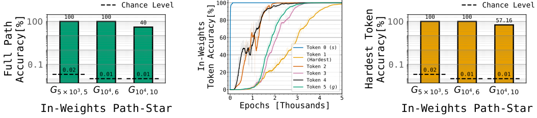
Figure 2: Success of Transformer in in-weights path-star task. (left) A next-token-trained Transformer achieves perfect or highly non-trivial accuracy on large path-star graphs G_{d,\ell} (Observation 1a). (middle) Learning order of tokens. The tokens of a path are not learned in the reverse order i.e., the model does not learn the right-to-left solution. Thus, gradients from the future tokens are not critical for success (Observation 1b). (right) Success of hardest-token-only task. In fact, the hardest token (the first) given the leaf is learned in isolation to non-trivial accuracy (Observation 1c). Success of this \ell -fold composition task is hard to explain within the associative memory view (§2.2). Analogous plots for Mamba are in Figure 7. We invite the reader to contrast these in-weights task results with the in-context task ones in Figure 4.
