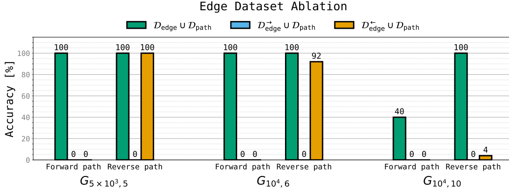
Figure 18: Mixed edge supervision enables forward path generation while forward-only fails due to reversal curse. Exact-match accuracy on held-out leaves for multiple path-star graphs (varying degree d and path length \ell ). As established, training on mixed edges \mathcal{D}_{\text{edge}} yields high non-trivial forward accuracy across graphs. But training on forward-only \mathcal{D}_{\text{edge}}^{\rightarrow} fails on both the forward and reverse tasks. This is indicative of the reversal curse. With backward-only edges ( \mathcal{D}_{\text{edge}}^{\leftarrow} ) the model attains high accuracy primarily on reverse path generation for smaller graphs. This can be reconciled by noting that generating the reverse path is an easier retrieval task. Random forward path accuracy is 1/d .
