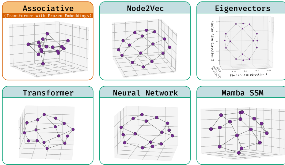
Figure 12: Tiny grid : Geometries of various architectures on a small 4 \times 4 grid graph. See Observation 4.
