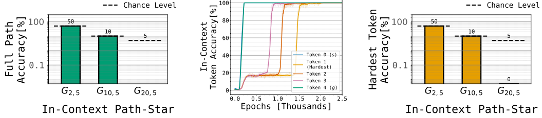
Figure 4: Failure of Transformer in in-context path-star task. We report the failure of next-token Transformers in the in-context version of the path-star task, reproducing results from B&N’24. (left) Full path accuracy remains at chance level across different small graph sizes. (Middle) Learning order of tokens with teacherless (multi-token-trained) objective shows a clear right-to-left learning cascade. (right) The hardest (first) token given the leaf fails to be learned in isolation, contrasting sharply with in-weights success shown in Figure 2.
