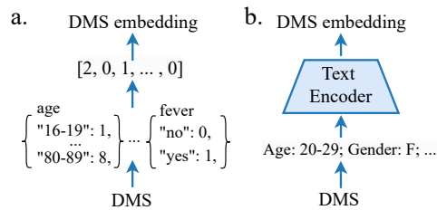
Figure 3: Existing DMS encoding methods.
