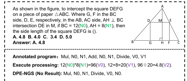
Figure 4: A typical case. A No Result type problem with a complex diagram.
