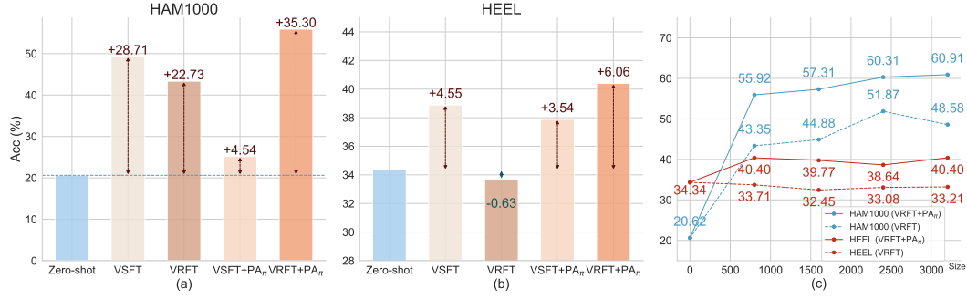
Figure 3: Performance comparison of different methods on the HAM10000 and HEEL. (a) and (b) show that VRFT + PA \pi achieves the highest accuracy, with a +35.30% improvement on HAM10000. (c) demonstrates that performance of VRFT + PA \pi improves with increasing training samples, reflecting enhanced perception capabilities. VSFT + PA \pi and VRFT + PA \pi are trained on bounding box prediction tasks (using SFT and GRPO, respectively) and evaluated on classification in a zero-shot manner, while V-SFT and V-RFT are directly trained for classification without localization.
