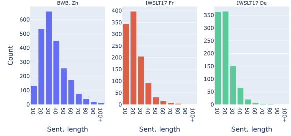
Figure 1: Sentence length distributions on test sets.
