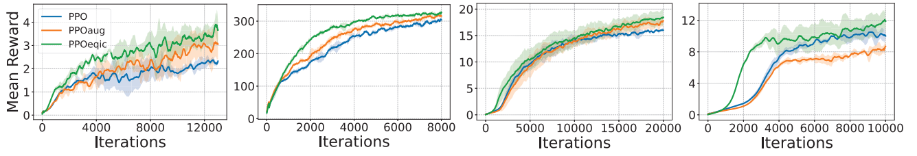
Fig. 3: Comparison of training curves of PPO, PPOaug, and PPOeqic on four tasks from left to right: Door Pushing, Dribbling, Stand Turning, and Slope Walking. Learning curves show mean episodic return and standard deviation for three seeds. PPOeqic consistently demonstrates the highest training returns and sample efficiency in all tasks.
