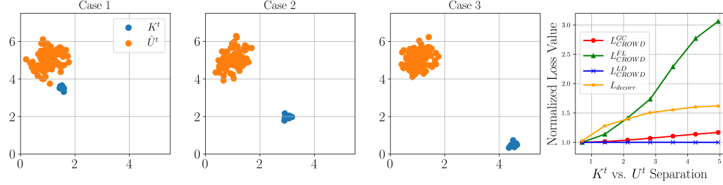
Figure 4: Characterization of losses in CROWD-L on a synthetic two-cluster imbalanced dataset by increasing known vs. unknown class separation (cases 1 through 3) similar to the RoI embedding space of h^t(\cdot; \theta) . The synthetic dataset generation is performed under the same seed.
