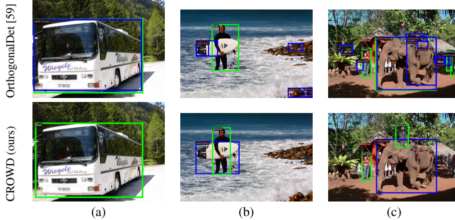
Figure 5: Qualitative results from CROWD contrasted against OrthogonalDet [59] showing that our approach mitigates (a) confusion (b) generalizes to unknowns and (c) reduces forgetting.
