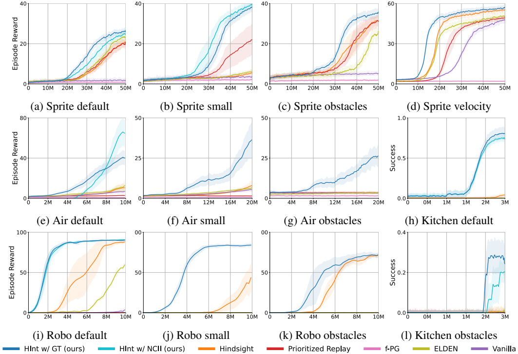
Figure 4: Comparison of HInt and HInt with NCII against baselines, 5 trials for each. HInt with NCII is used in Spriteworld default, small, Robosuite default, Air Hockey default, Kitchen default, and obstacles. The shading indicates standard error. X axis is the number of timesteps.
