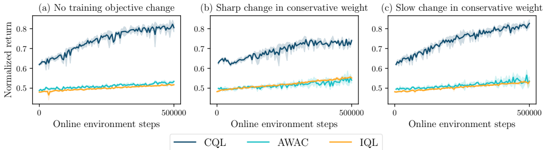
Figure 3: Comparison of results for online fine-tuning on halfcheetah-medium-v2 for CQL, AWAC, and IQL for 3 settings: (1) fine-tuning with the same offline training objective, (2) immediately changing the training objective to be less conservative at the online phase, and (3) linearly changing the hyper-parameters to make the training objective less conservative. For CQL we reduce the Lagrange threshold from 5 to 0.5, for AWAC we reduce the Lagrange multiplier from 1 to 0.1, and for IQL we increase the expectile from 0.7 to 0.85.
