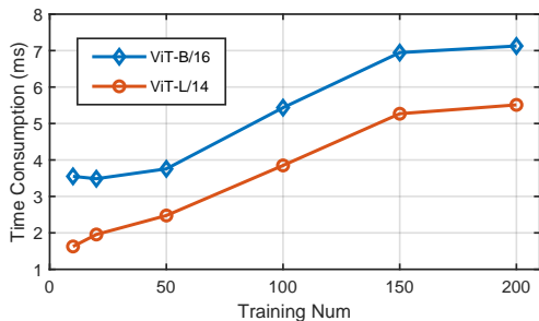
Figure 5: Time consumption of the optimization phase of our MADA approach, based on both CLIP ViT-B/16 and CLIP ViT-L/14 respectively on VOC dataset. MADA optimization solution achieves considerable efficiency (millisecond-level) compared with other optimization methods.
