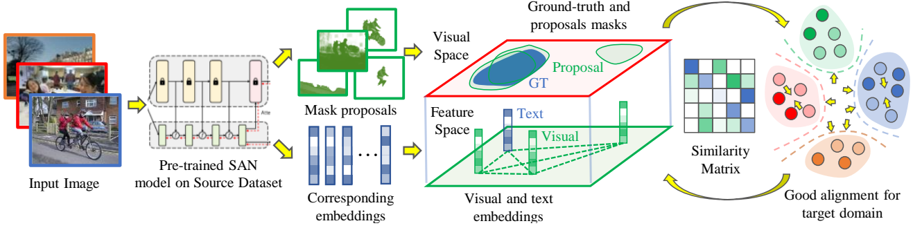
Figure 2: Framework of our MADA approach. Image samples are set as inputs to raw segmentation models (e.g., SAN). Then, both the visual masks as well as the corresponding feature representations are obtained. We assume the more similar of the predicted masks compared with the ground truth, the more similar the feature representation is. To this end, MADA jointly explores the similarities of masks and representations, aligning the shift in both source and target domains.
