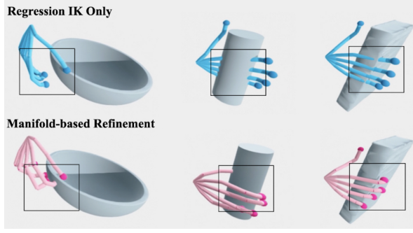
Fig. 6: Qualitative comparison before and after applying hand motion refinement model for synthetic data generation.
