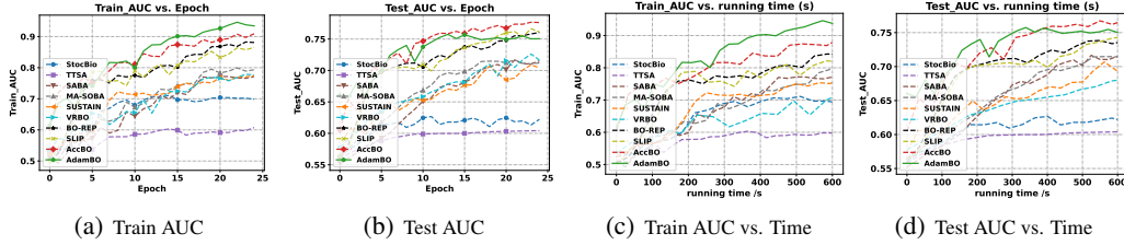
Figure 4: RNN for AUC maximization on Sentiment140 dataset with imbalance ratio of 0.8. Figures (a), (b) are the results over epochs, Figures (c), (d) are the results over running time.
