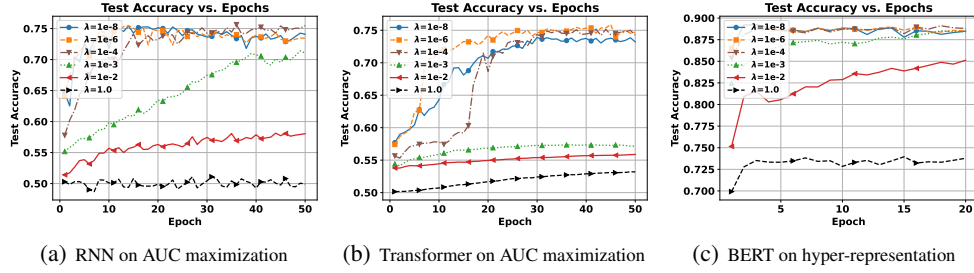
Figure 5: Test accuracy of different models on AUC maximization and hyper-representation using AdamBO with \beta = 0.1 , \beta_{sq} = 0.001 and different \lambda s. (a) a 2-layer RNN model on AUC maximization (data imbalanced ratio = 0.8); (b) a 2-layer Transformer model on AUC maximization (data imbalanced ratio = 0.9); (c) an 8-layer BERT model on hyper-representation.
