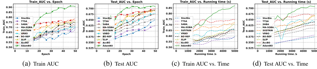
Figure 2: Transformer for AUC maximization on Sentiment140 dataset with imbalance ratio of 0.9.
