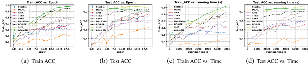
Figure 3: Comparison with bilevel optimization baselines on RNN for hyper-representation.
