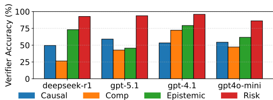
Figure 4: Verifier accuracy across reasoning families and models.
