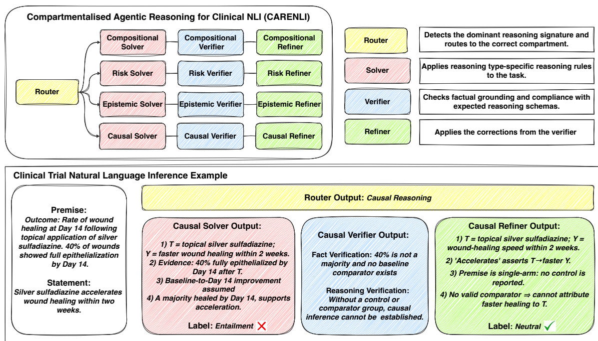
Figure 1: CARENLI: Compartmentalised agentic reasoning framework for Clinical Trial NLI . A Router assigns each premise–statement pair to a dominant reasoning type (Causal Attribution, Compositional Grounding, Epistemic Verification, or Risk State Abstraction). A reasoning-type-specific solver produces a provisional NLI label and explicit reasoning trace, which a verifier audits for factual grounding and schema compliance, and a refiner minimally corrects when needed. The figure illustrates the pipeline on a causal attribution example. Unlike generic prompting strategies CARENLI enforces formalised, structured reasoning trajectories that are explicitly grounded in clinical trial semantics and checked for logical consistency.
