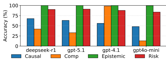
Figure 3: Overall accuracy of reasoning classification across models.
