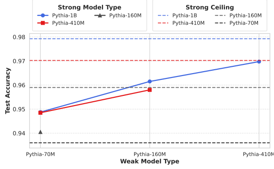
(a) Accuracy (Pythia).
