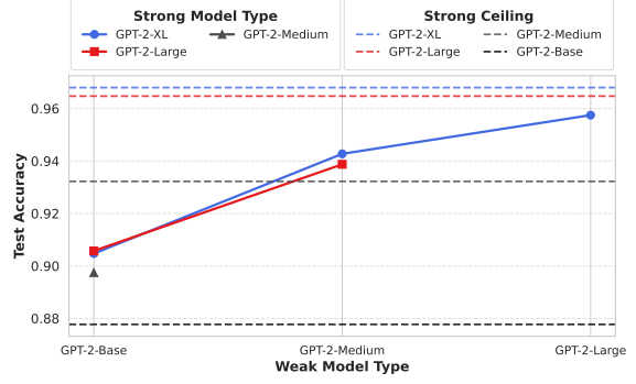
(b) Accuracy (GPT-2).
