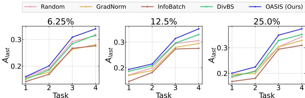
Figure 5: Average accuracies over time on COAST benchmark under different selection ratios. Performance at task t denotes the average accuracy over all seen tasks up to that point ( i.e. , task 1 through task t ). We use LLaVA-1.5-7B as the model across all selection ratios.
