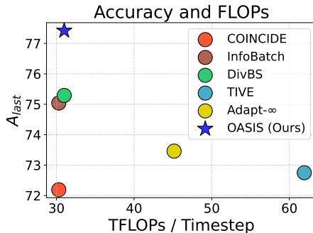
Figure 3: Accuracy and FLOPs with 25% selection ratio on MICVIT. The top-left corner shows effective and efficient sample selection.
