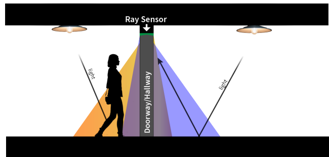
Figure 1: The overall system concept of Ray, a batteryless, energy-harvesting, doorway mounted occupancy tracking and person detection enabling system. This system uses reflective indoor lighting to both power the system and detect person entry and exit activity to a room or corridor.
