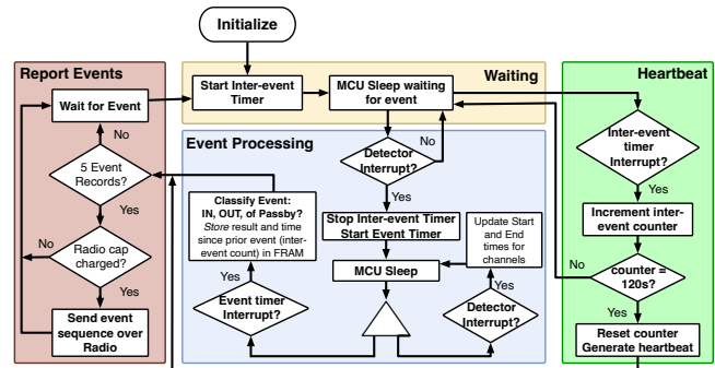
Figure 4: The Ray detection algorithm and system decision flowchart. The algorithm is composed of four parts that handle reporting doorway events, processing detected events, processing time between events and heartbeats, and idle waiting.
