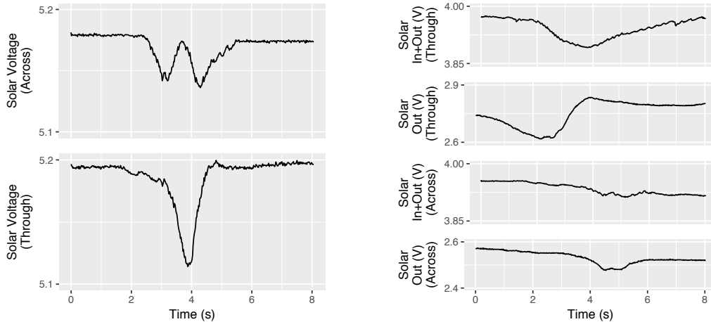
(a) These traces show the solar panel output in the presence of the “Spotlight” effect. The top figure shows the response when someone walks across the “Spotlight”, while the bottom one shows the response when someone walks through the door.
