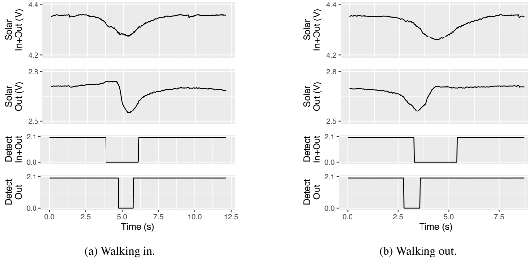
Figure 3: These traces show example solar panel voltages and detector outputs over time when a person walks through a Ray-enabled doorway. The top traces show how the solar panel’s voltages are deformed during the doorway event. The detector triggers are used to wake up the microcontroller and detect events and their direction. The angling of the panels cause the inward facing and outward facing detectors to trigger at different times depending on the direction the person is walking.
