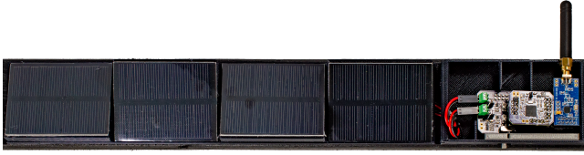
Figure 5: 3D printed solar panel and PCB housing enclosure with angled slots for solar energy harvesters and the Ray prototype PCB.
