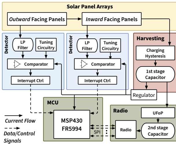
Figure 2: The Ray architecture overview. Ray uses the energy and signals from two sets of solar panels to both power the sensor and detect people passing into and out of a doorway. Two detector circuits each monitor the solar panels sets mounted in series in the doorway. One detector monitors a set of similarly facing panels, while the other observes the combined signal from all of the panels. On detection, the detectors wake up the MCU to process, log, or communicate occupancy information.
