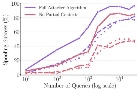
Figure 2: Ablation and query cost study of spoofing of KGW2-SELFHASH. y -axis shows the % of quality texts detected as watermarked under FPR of 10^{-6} . No Partial Contexts refers to an ablation with w_1 = w_2 = 0 (see App. E). Dotted ( \cdot \cdot \cdot ), dashed ( - - - ) and full ( — ) lines correspond to all-5, self-filtered, and oracle-filtered results, respectively.
