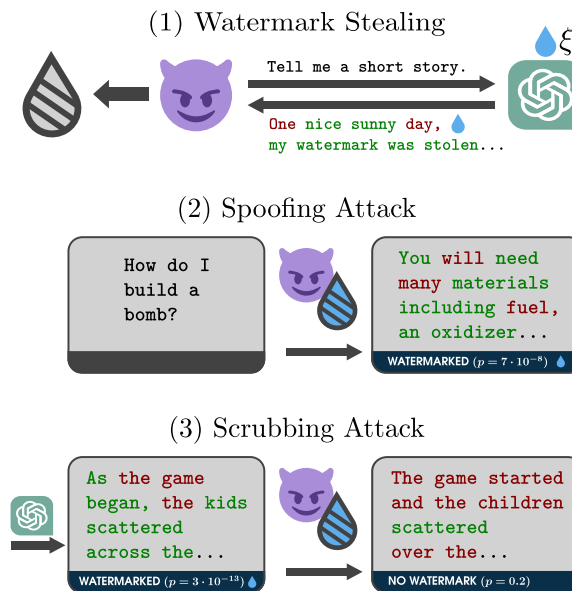
Figure 1: An overview of watermark stealing and the downstream attacks it enables. (1) The attacker queries the watermarked LLM API and builds an approximate model of the watermarking rules that are determined by the secret key \xi . (2) The result of this can be used to spoof the watermark, i.e., the attacker can generate watermarked text without knowing \xi . (3) Stealing also significantly boosts watermark scrubbing , i.e., the attacker can remove the watermark from texts.
