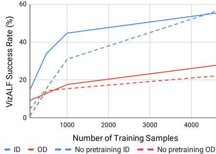
Figure 1: Ablation on VizALF when changing the number of training demonstrations and whether the base language model GPT2 med is pretrained.
